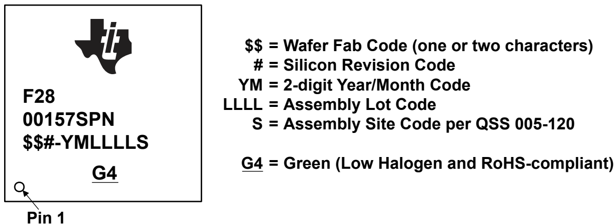
Figure 9-2. Package Symbolization for PN Package
