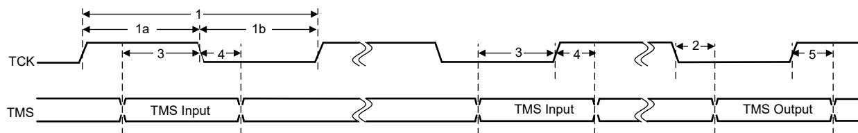
Figure 6-23. cJTAG Timing
