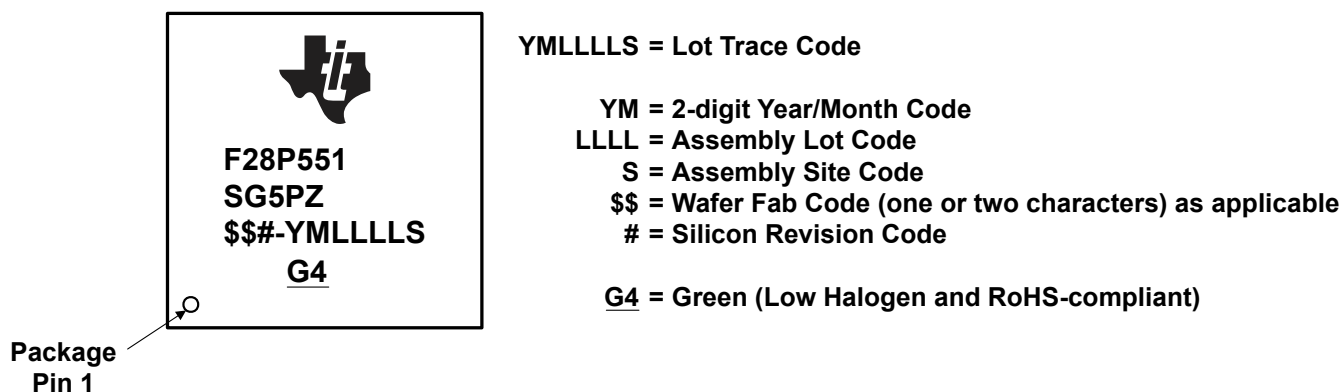
Figure 9-7. Package Symbolization for PZ Package – Non-Automotive
