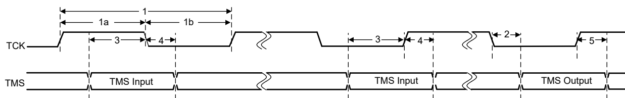
Figure 6-25. cJTAG Timing
