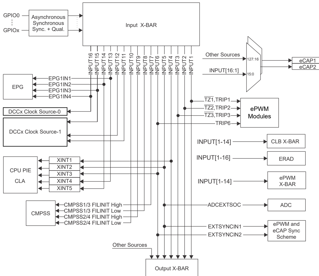
Figure 5-9. Input X-BAR
