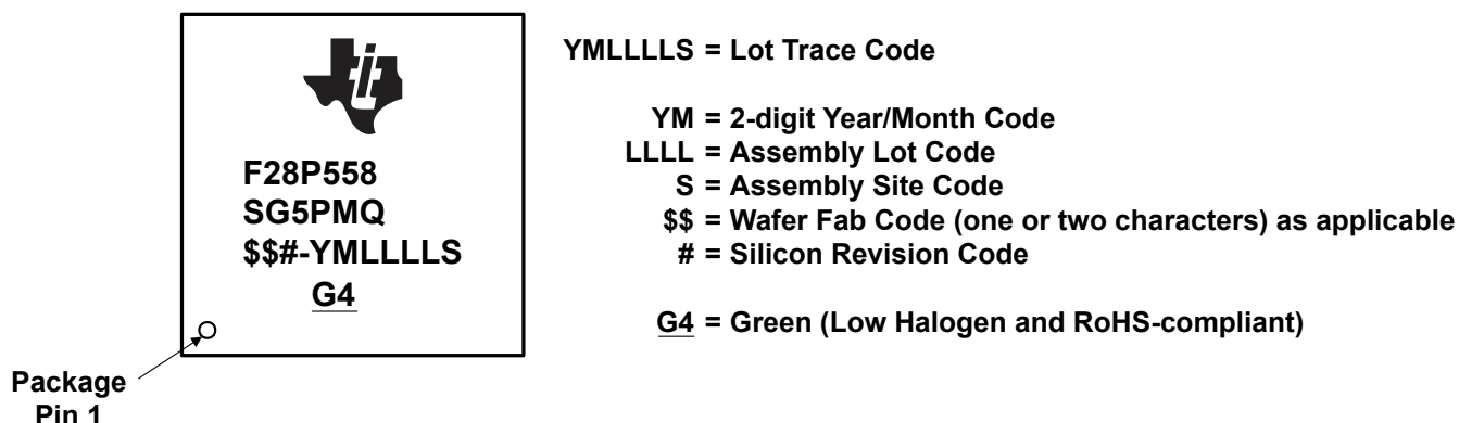
Figure 9-6. Package Symbolization for PM Package – Automotive
