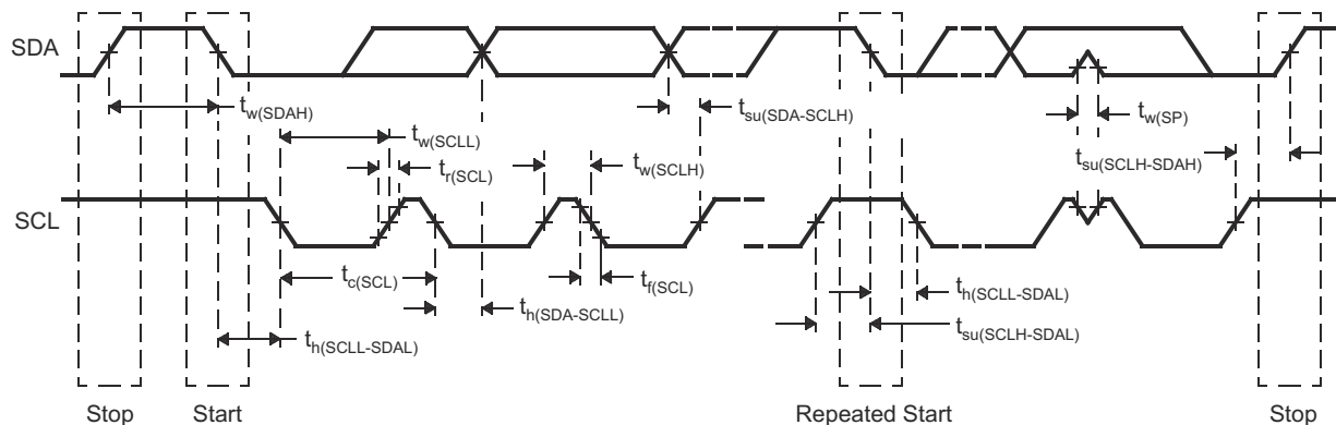
Figure 8-19. I2C Timings
