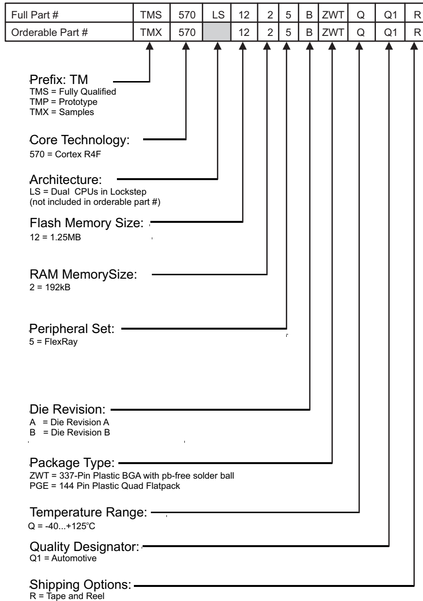
Figure 8-1. TMS570LS1225 Device Numbering Conventions
