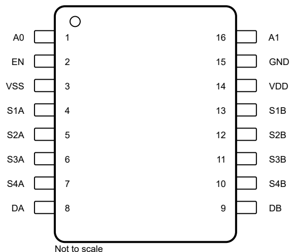
Figure 4-1. PW Package, 16-Pin TSSOP (Top View)
