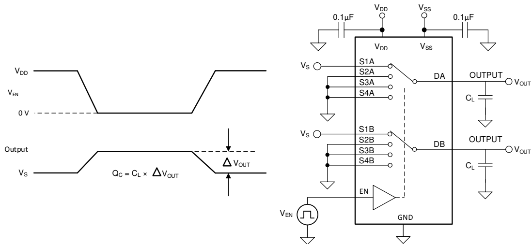
Figure 6-7. Charge-Injection Measurement Setup
