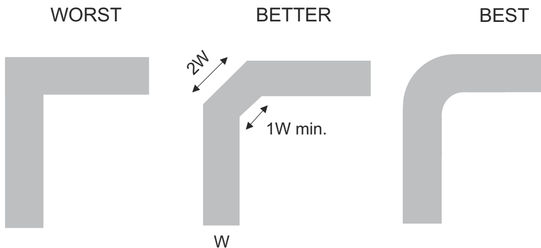
Figure 8-3. Trace Example
