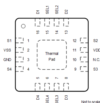
Figure 5-2. RUM Package 16-Pin WQFN Top View
