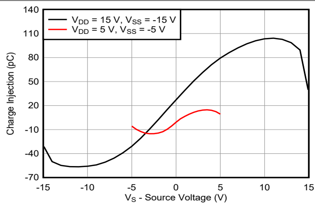
Figure 5-14. Charge Injection vs Source Voltage – Dual Supply
