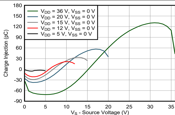
Figure 5-16. Charge Injection vs Source Voltage – Single Supply
