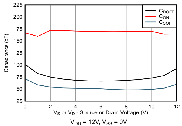
Figure 5-26. Capacitance vs Source or Drain Voltage
