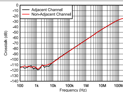
Figure 6-24. Crosstalk vs Frequency
