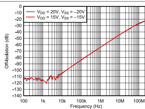
Figure 6-22. Off-Isolation vs Frequency
