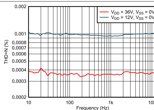
Figure 6-24. THD+N vs. Frequency (Single Supplies)
