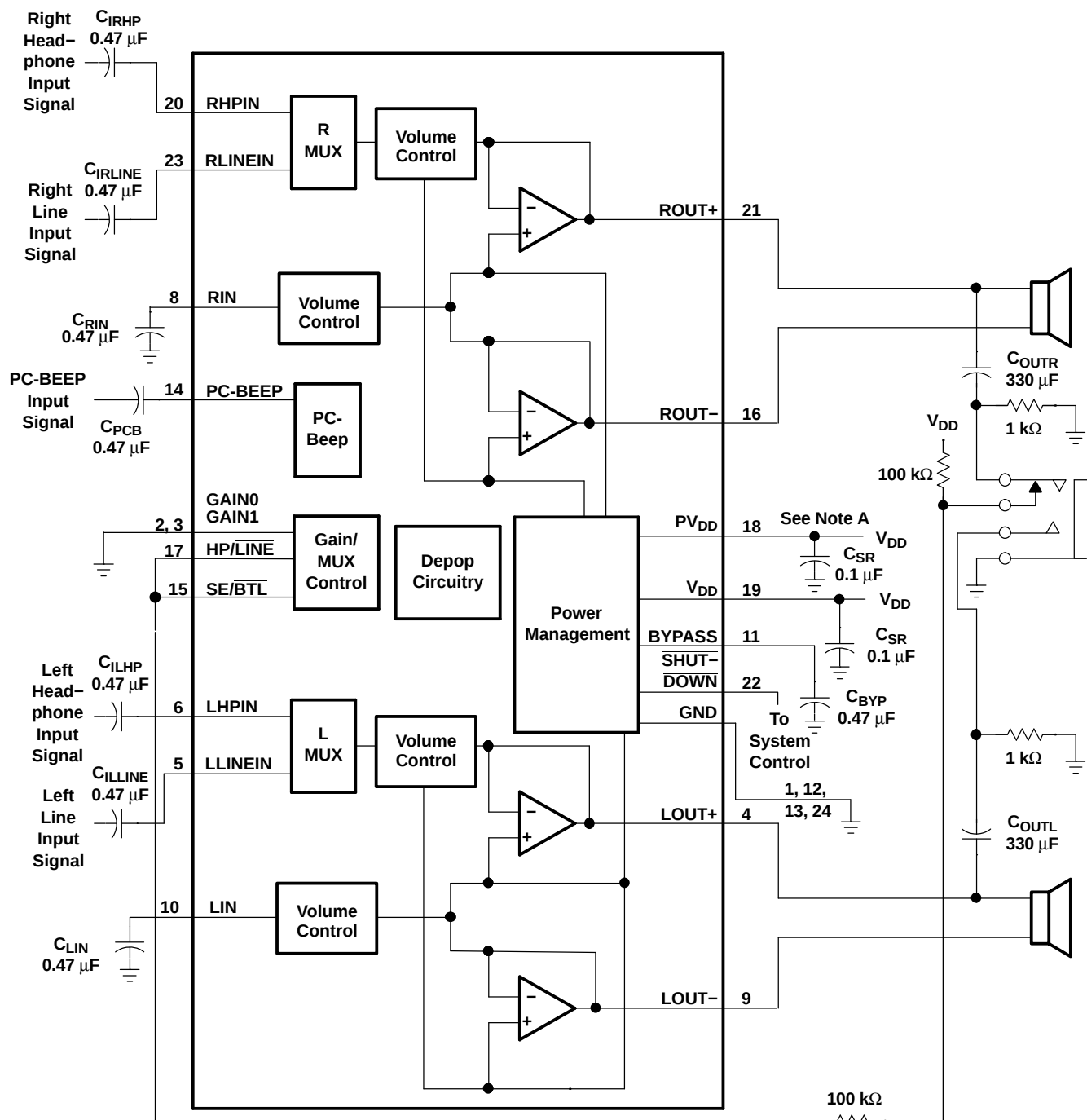
Figure 37. Typical TPA0312 Application Circuit Using Single-Ended Inputs and Input MUX
