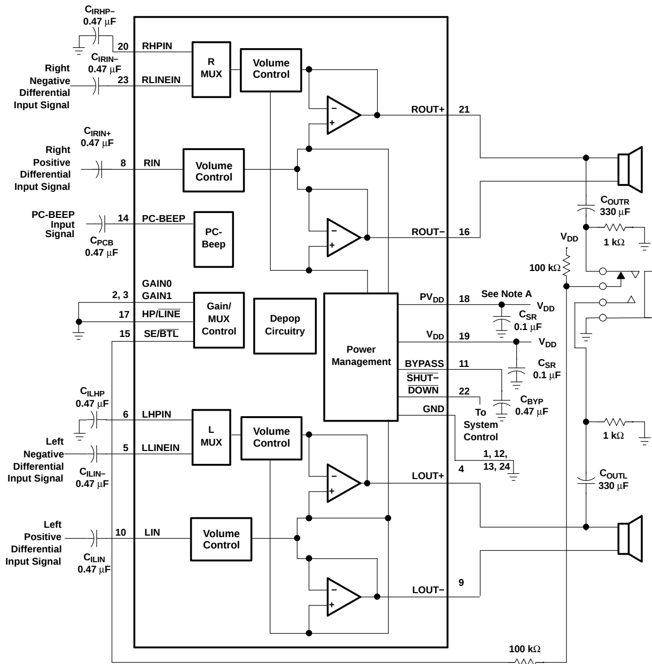
Figure 38. Typical TPA0312 Application Circuit Using Differential Inputs
