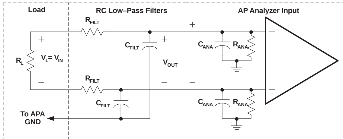
Figure 51. Measurement Low-Pass Filter Derivation Circuit—Class-D APAs
