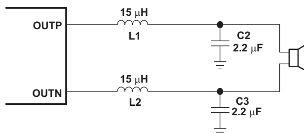
Figure 34. Typical LC Output Filter, Cutoff Frequency of 27 kHz, Speaker Impedance = 4 Ω
