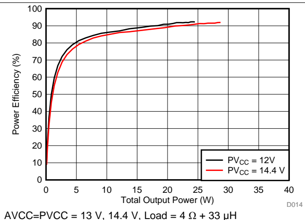
Figure 16. Efficiency vs Output Power (PBTL)
