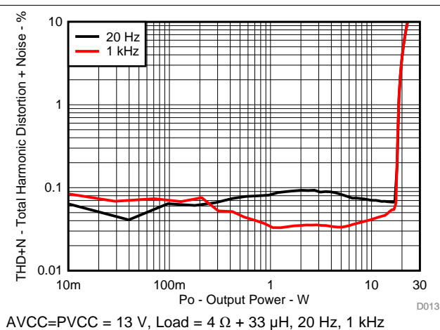
Figure 14. THD+N vs Output Power (PBTL)
