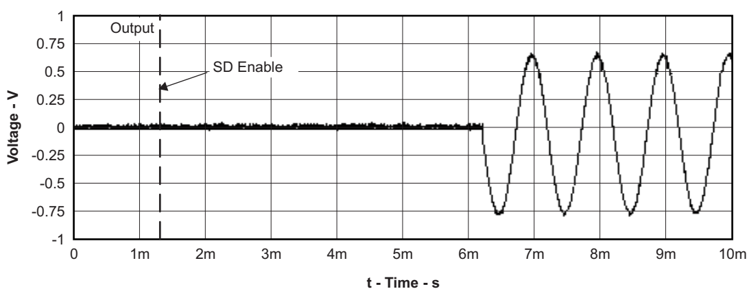
Figure 23. Startup Time
