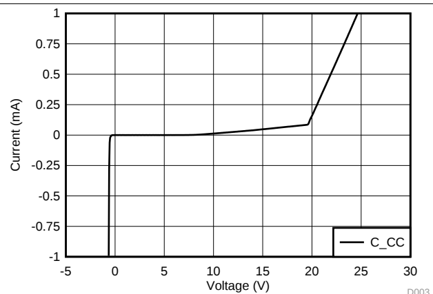
Figure 24. C_CC IV Curve
