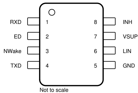
Figure 6-1. D Package, 8-Pin SOIC
