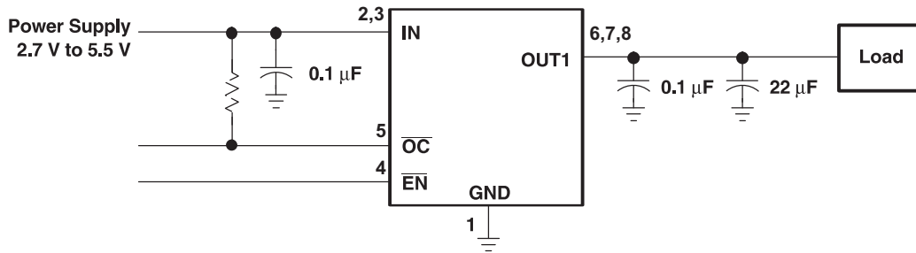
Figure 6. Typical Application
