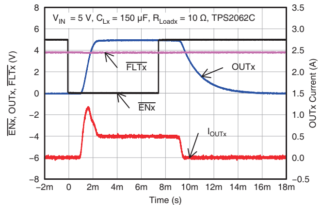
Figure 12. TPS2062C Enable and Disable into 10- \Omega Load
