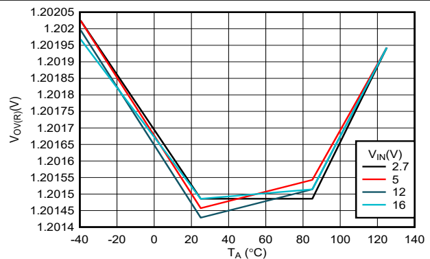
Figure 6-11. EN/UVLO Rising Threshold vs Temperature
