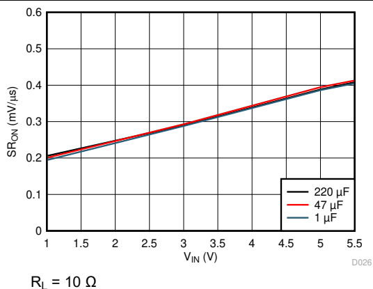
Figure 7-23. Slew Rate vs Load Capacitance ( C_T = 10000\text{ pF} )
