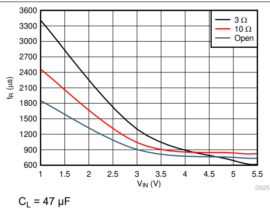
Figure 7-22. Rise Time vs Load Resistance ( C_T = 10000\text{ pF} )
