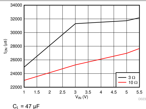
Figure 7-20. Turn-On vs Load Resistance ( C_T = 10000\text{ pF} )
