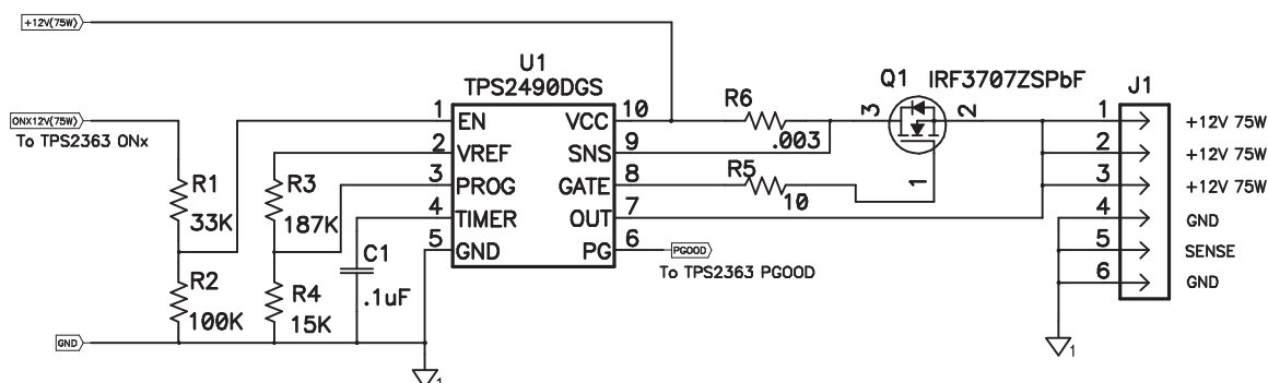
Figure 8. 150-W Application
