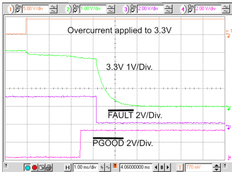
Figure 15. Over Current Applied to 3.3 V - \overline{\text{FAULT}} & \overline{\text{PGOOD}}
