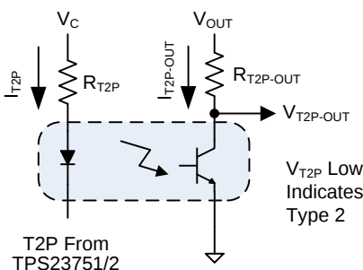
Figure 35. T2P Interface
