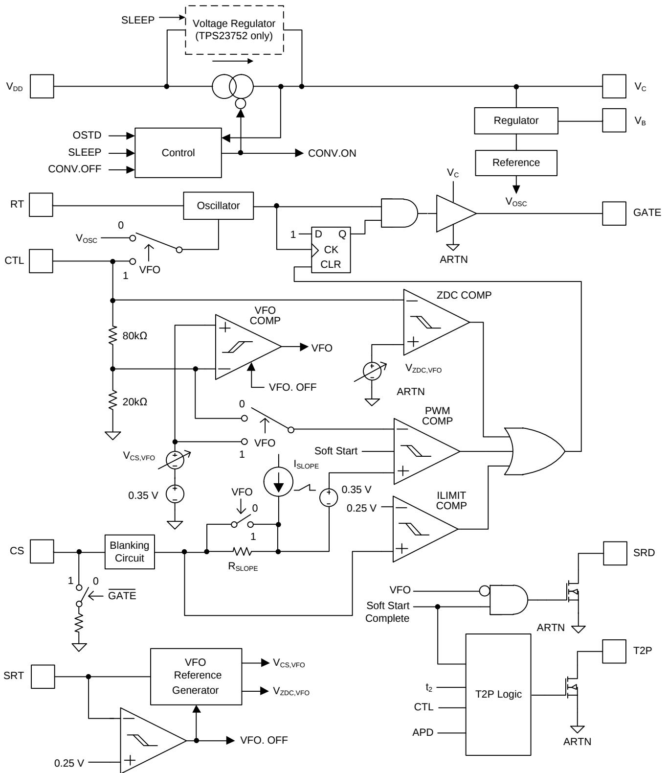
Figure 20. DC-DC Controller
