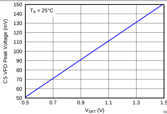
Figure 7. CS VFO Peak Voltage vs SRT Voltage
