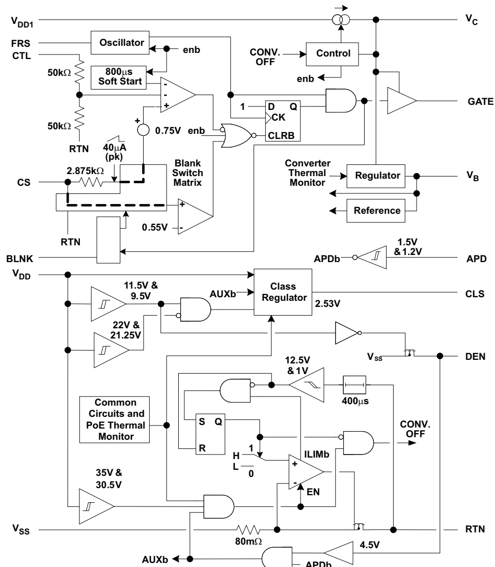
Figure 2. TPS23753 Functional Block Diagram
