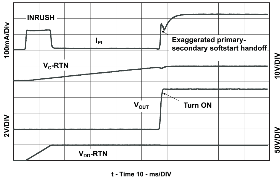
Figure 19. Power Up and Start
