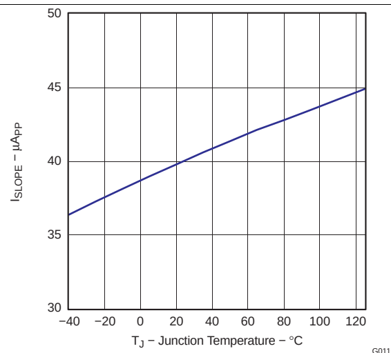
Figure 15. Current Slope Compensation Current vs Temperature
