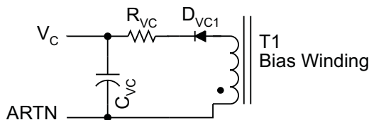
Figure 29. R_{VC} Usage
