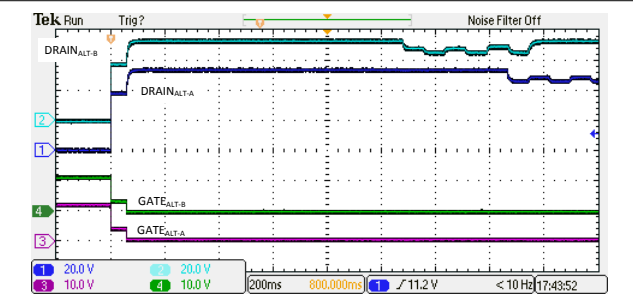
Figure 9-7. 4-Pair Backoff Due to I_{LIM} Fault
