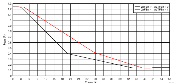
Figure 8-57. 2x Mode ( 2xFBn = 1 ) Foldback Curves, I_{PORT} vs V_{DRAIN}
