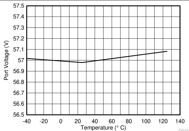
Figure 6-15. Port Voltage ADC Measurement vs Temperature
