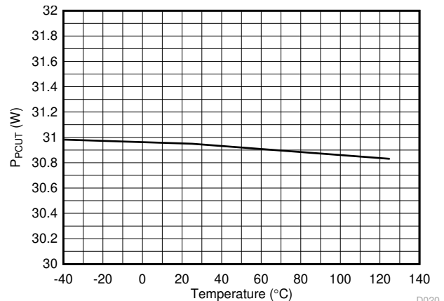
Figure 6-20. 2-Pair PCut Threshold (30W) vs Temperature
