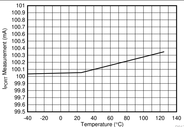
Figure 6-17. Port Current ADC Measurement (100mA) vs Temperature
