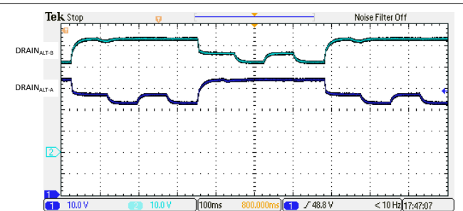
Figure 9-13. 4-Pair High Resistance (36kΩ) Detection Signature
