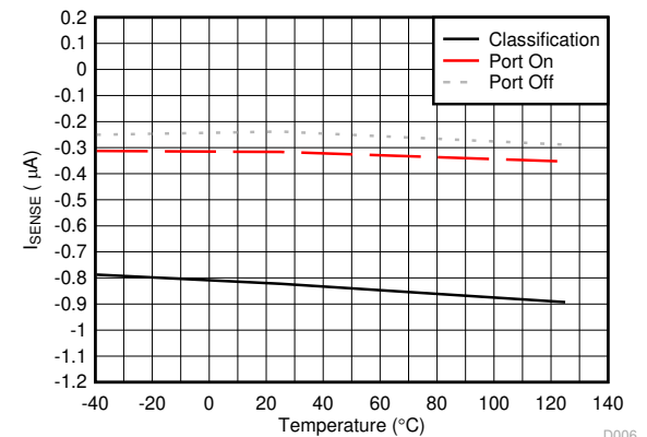
Figure 6-6. SENSE Pin Bias Current vs Temperature
