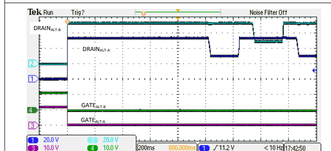
Figure 9-8. 4-Pair Backoff Due to 4PPCut Fault
