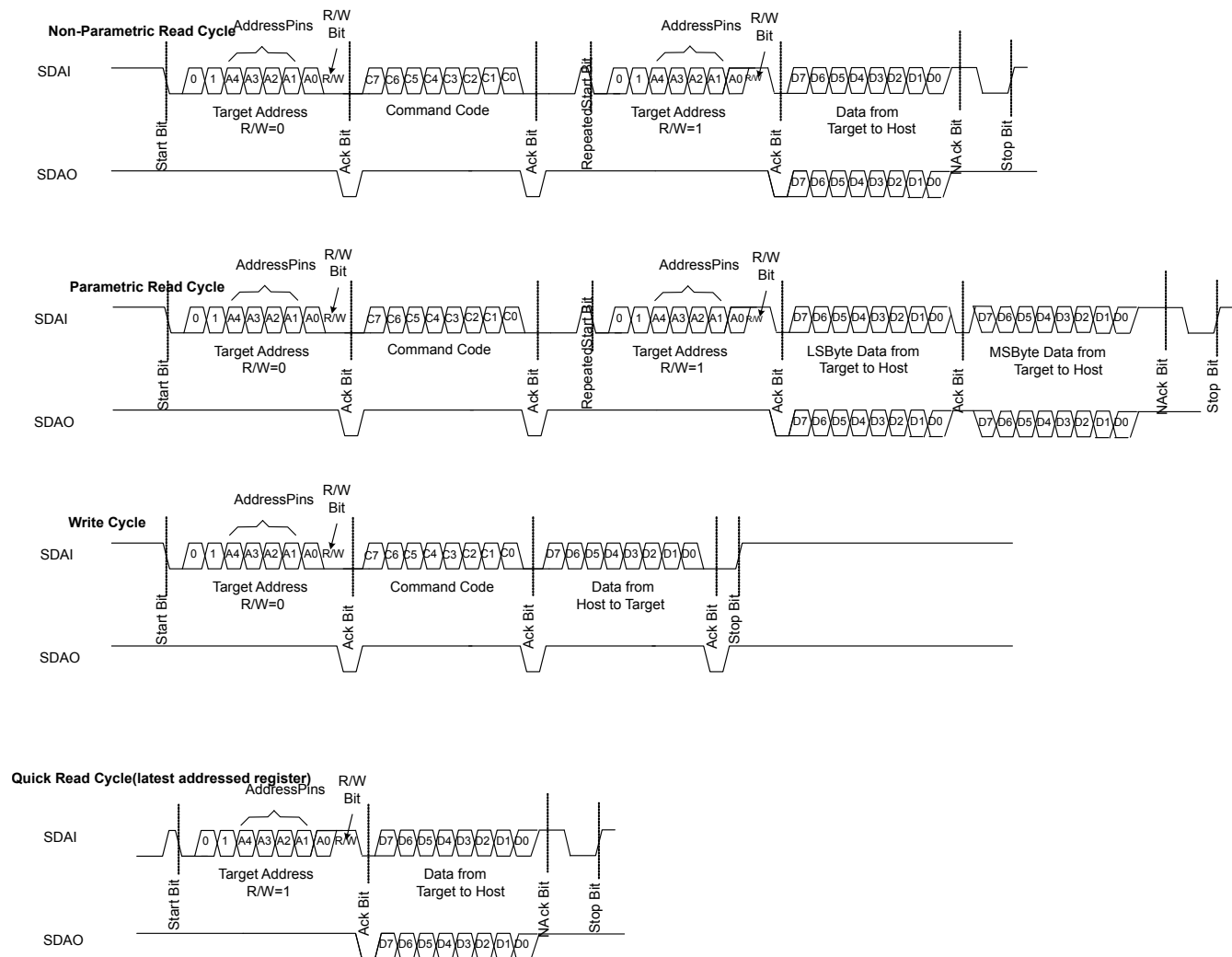
Figure 8-6. I 2 C interface Read and Write Protocol – Configuration A
