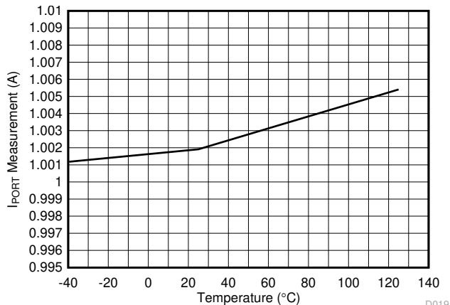
Figure 6-19. Port Current ADC Measurement (1 A) vs Temperature
