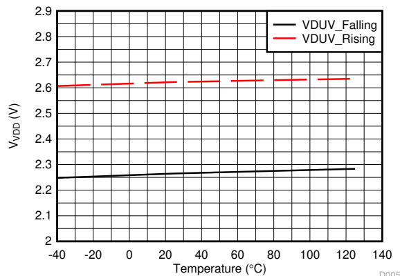
Figure 6-5. VDUV Thresholds vs Temperature
