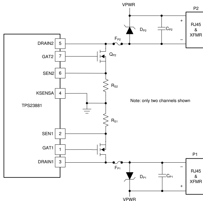
Figure 9-28. Kelvin Current-Sense Connection
