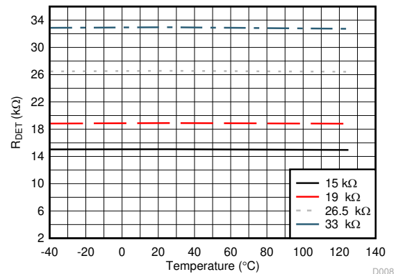
Figure 6-8. Discovery Resistance Measurement vs Temperature
