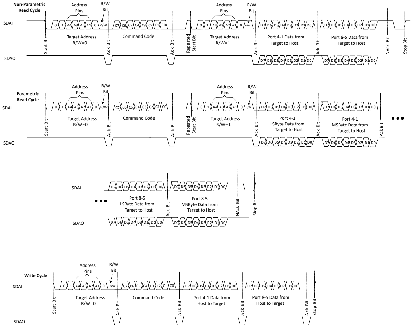
Figure 8-7. I 2 C interface Read and Write Protocol – Configuration B
