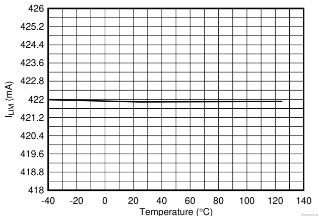
Figure 6-24. 1x Mode (2xFBn = 0) Current Limit vs Temperature
