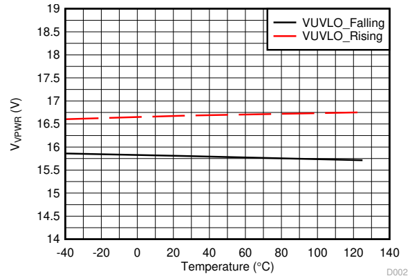
Figure 6-2. VPWR UVLO Thresholds vs Temperature
