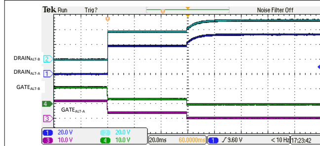
Figure 9-6. 4-Pair I_{LIM} Foldback and Turn Off
