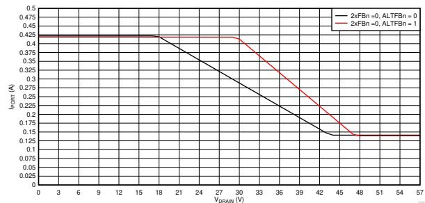
Figure 8-79. 1x Mode (2xFBn = 0) Foldback Curves, I_{PORT} vs V_{DRAIN}
