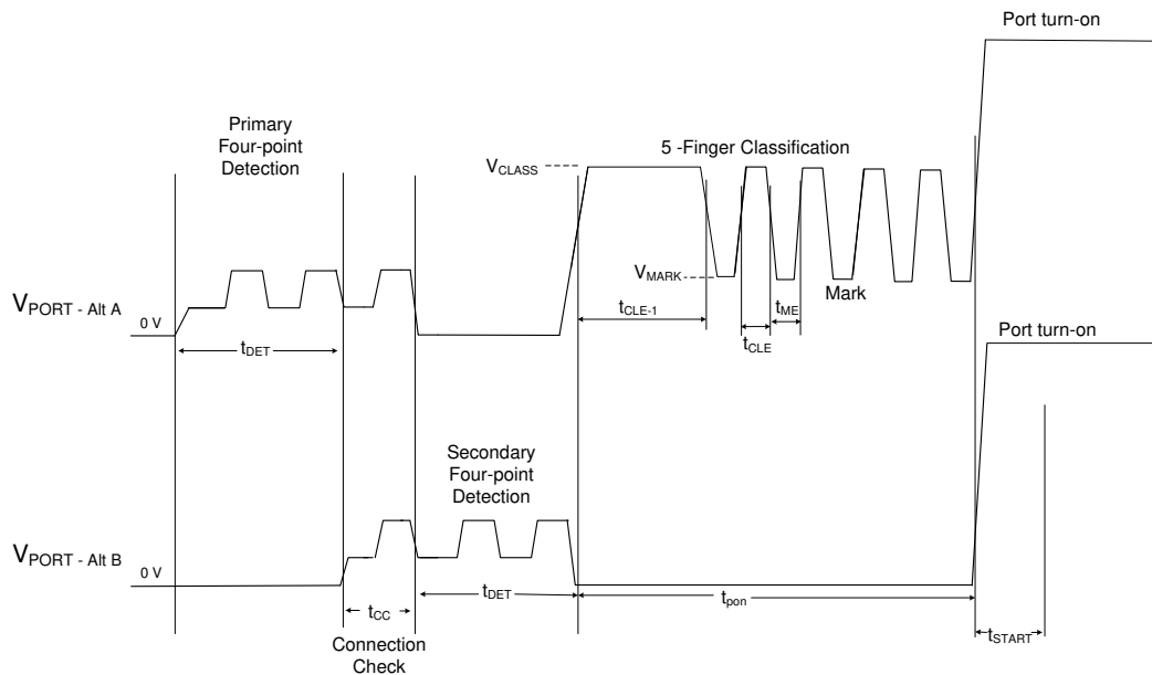
Figure 7-6. 4-Pair Single Signature Detection, 5-Event Classification and Turn-On
