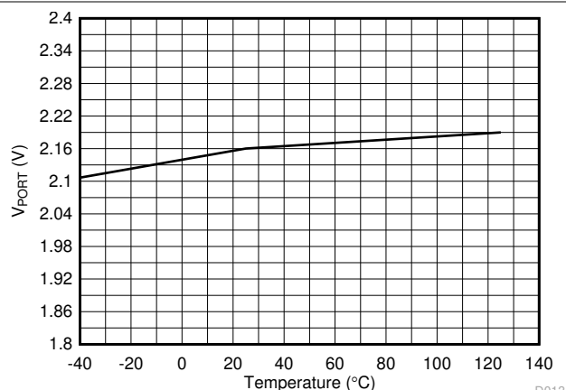
Figure 6-13. Power Good Threshold vs Temperature
