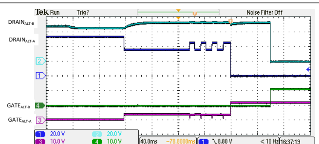
Figure 9-21. 4-Pair Single Signature 4-Finger Classification and Turn On
