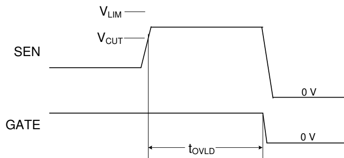
Figure 7-2. Overcurrent Fault Timing
