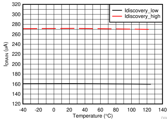
Figure 6-7. Discovery Currents vs Temperature
