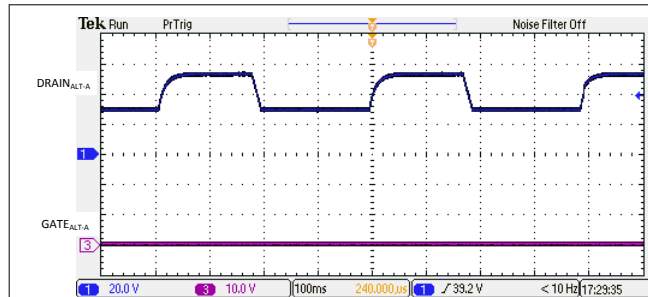
Figure 9-10. 2-Pair Open Circuit Detection Signature
