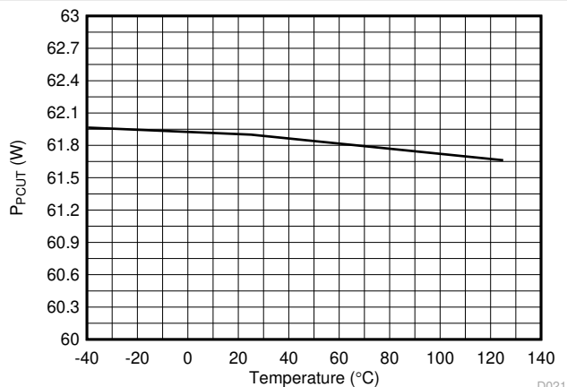
Figure 6-21. 4-Pair PCut Threshold (60W) vs Temperature
