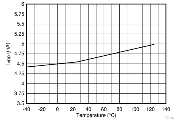
Figure 6-4. VDD Current Consumption vs Temperature
