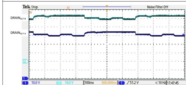
Figure 9-12. 4-Pair Low Resistance (11kΩ) Detection Signature
