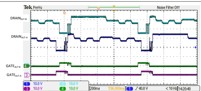
Figure 9-23. 4-Pair Semi-Auto Mode Discovery with a Valid Dual Signature Class 4D Load
