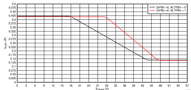
Figure 8-56. 1x Mode ( 2xFBn = 0 ) Foldback Curves, I_{PORT} vs V_{DRAIN}
