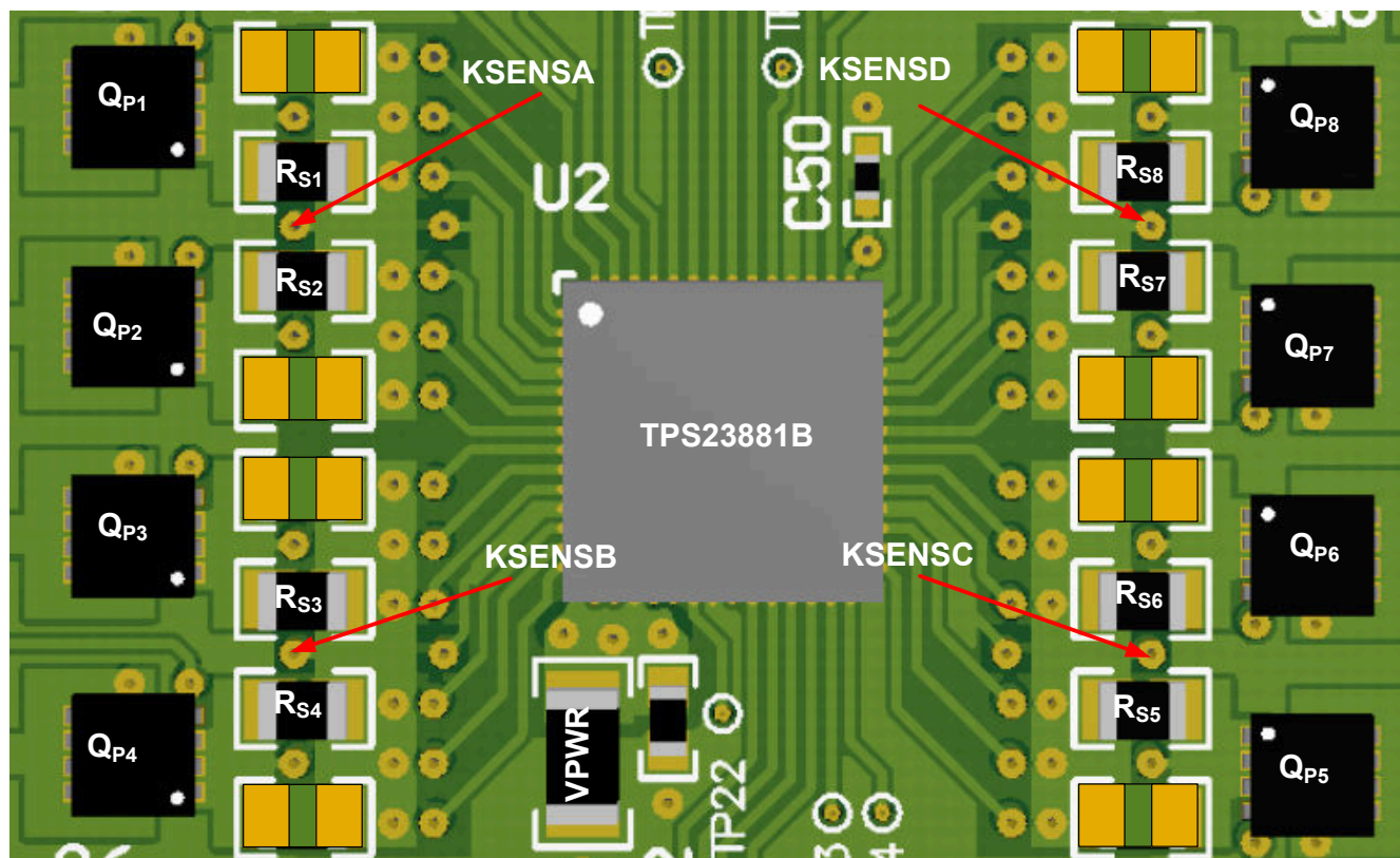
Figure 9-30. Eight Port Layout Example (Top Side)
