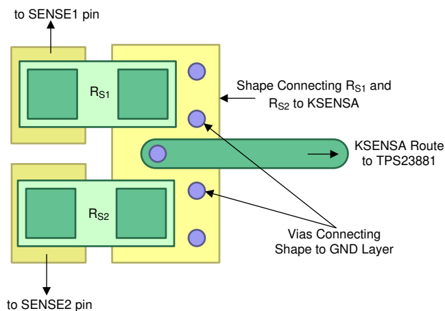
Figure 9-29. Kelvin Sense Layout Example
