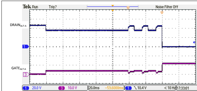
Figure 9-16. 2-Pair 3-Finger Classification and Turn-On
