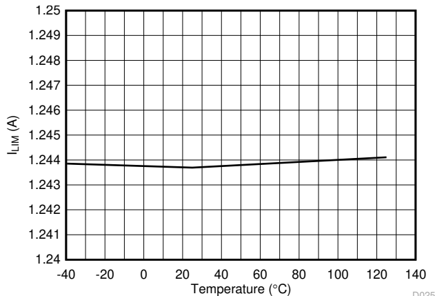
Figure 6-25. 2x Mode (2xFBn = 1) Current Limit vs Temperature
