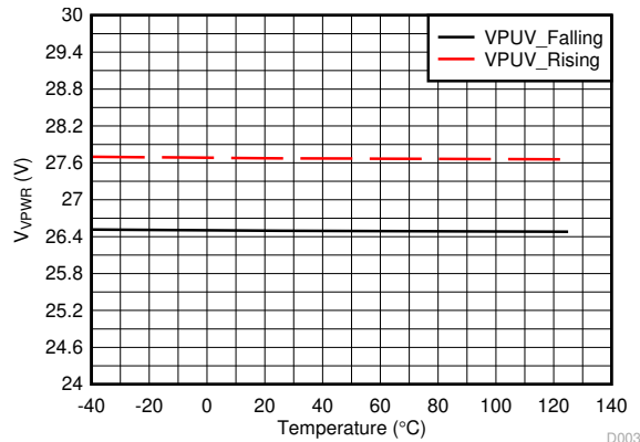
Figure 6-3. VPUV Thresholds vs Temperature
