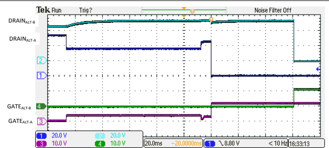
Figure 9-19. 4-Pair Single Signature 1-Finger Classification and Turn On
