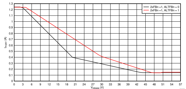
Figure 8-80. 2x Mode (2xFBn = 1) Foldback Curves, I_{PORT} vs V_{DRAIN}
