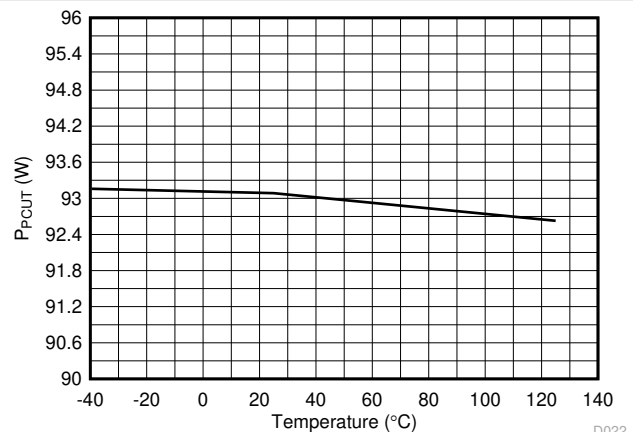
Figure 6-22. 4-Pair PCut Threshold (90W) vs Temperature
