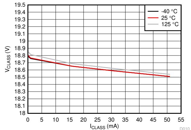
Figure 6-10. Classification Voltage vs I_{CLASS} and Temperature
