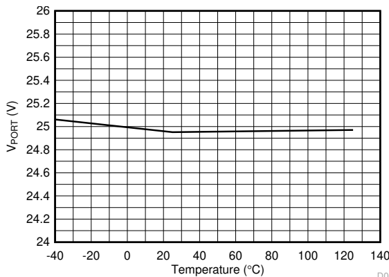
Figure 6-9. Discovery Open Circuit Voltage vs Temperature
