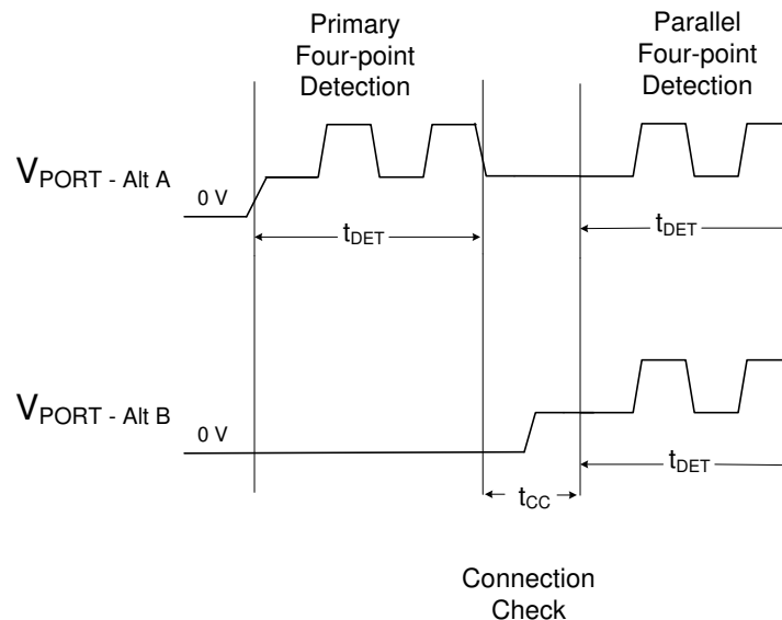
Figure 8-5. 4-Pair Port, Detection and Connection Check Waveforms with a Dual Signature Load
