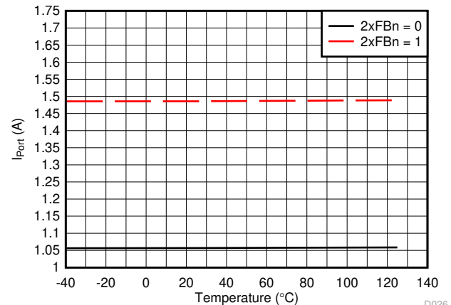
Figure 6-26. I_{\text{SHORT}} Threshold vs Temperature
