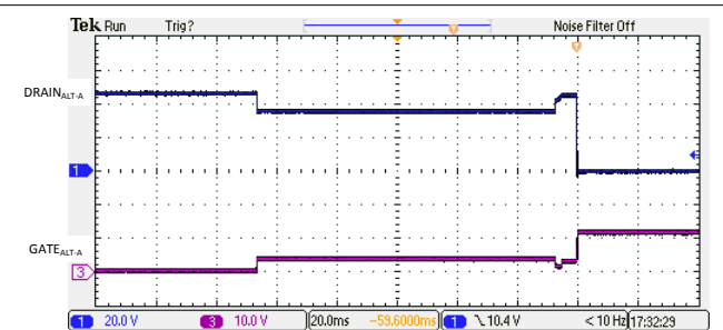
Figure 9-15. 2-Pair 1-Finger Classification and Turn-On
