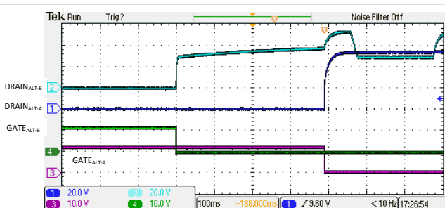
Figure 9-9. 4-Pair Single Signature Class 0-4 Disconnect
