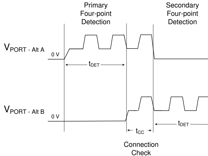
Figure 8-4. 4-Pair Port, Detection and Connection Check Waveforms with a Single Signature Load
