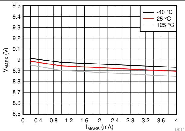
Figure 6-11. Mark Voltage vs I_{MARK} and Temperature
