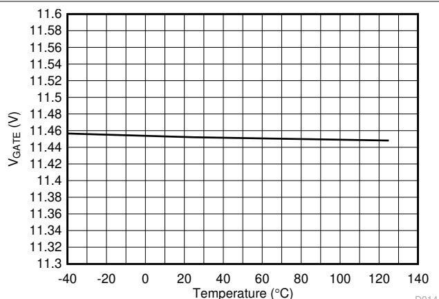
Figure 6-14. Gate Voltage (Port On) vs Temperature
