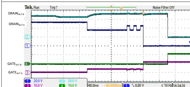
Figure 9-20. 4-Pair Single Signature 3-Finger Classification and Turn On
