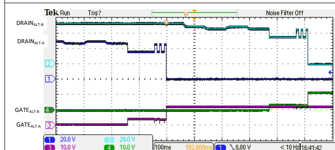
Figure 9-26. 4-Pair Dual Signature 3-Finger Classification and Turn On
