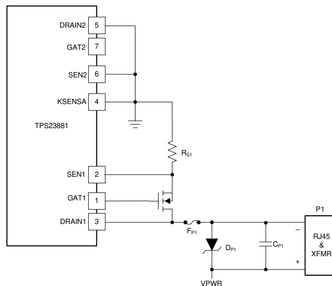
Figure 9-3. Unused PORT2 Connections
