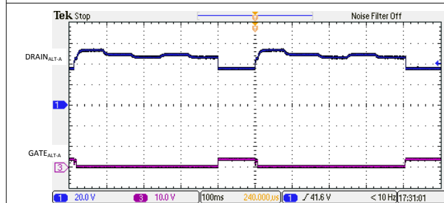
Figure 9-14. 2-Pair Semiauto Mode Discovery with a Valid Class 0-3 Load
