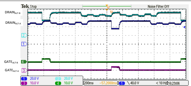
Figure 9-17. 4-Pair Semi-Auto Mode Discovery with a Valid Single Signature Class 0-3 Load
