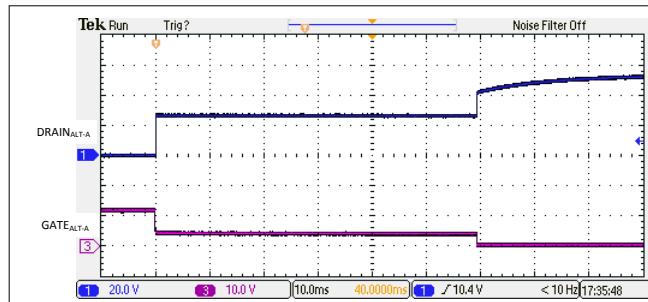
Figure 9-4. 2-Pair I_{LIM} Foldback and Turn-Off
