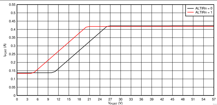
Figure 8-81. Inrush Foldback Curves, I_{PORT} vs V_{PORT}
