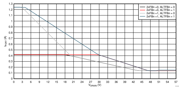
Figure 8-3. Foldback When the Port is Already ON: I_{LIM} vs V_{drain}
