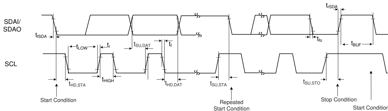
Figure 7-1. I 2 C Timings
