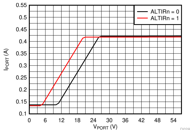
Figure 6-28. Inrush Current Foldback vs Port Voltage
