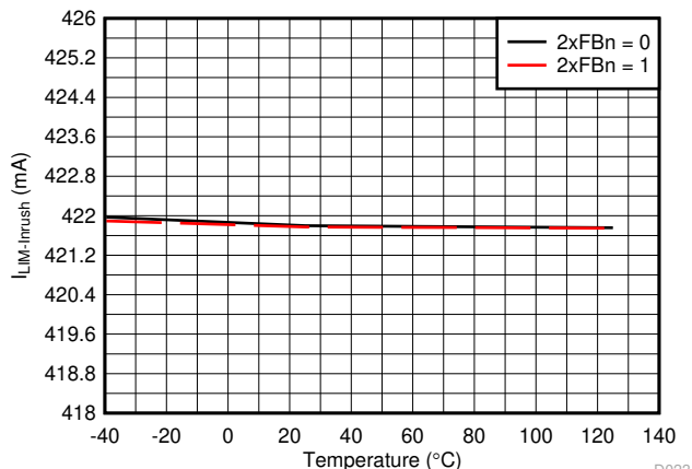
Figure 6-23. Inrush Current Limit vs Temperature
