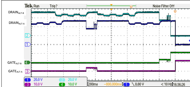
Figure 9-18. 4-Pair Single Signature Discovery and Turn On from Semi-Auto Mode
