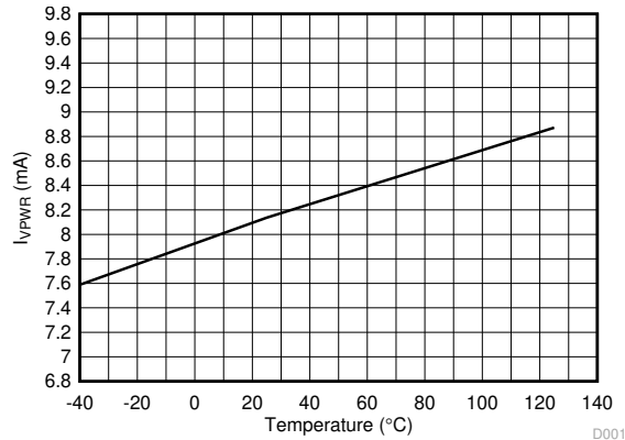
Figure 6-1. VPWR Current Consumption vs Temperature
