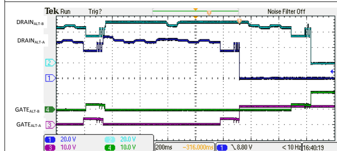
Figure 9-24. 4-Pair Dual Signature Discovery and Turn On from Semi-Auto Mode
