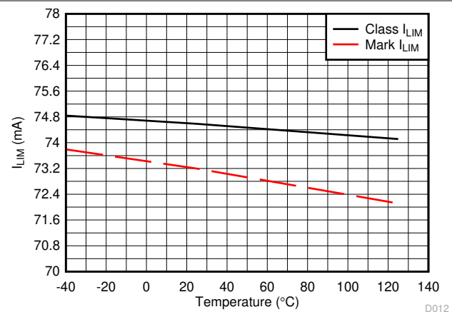
Figure 6-12. Classification and Mark Current Limit vs Temperature
