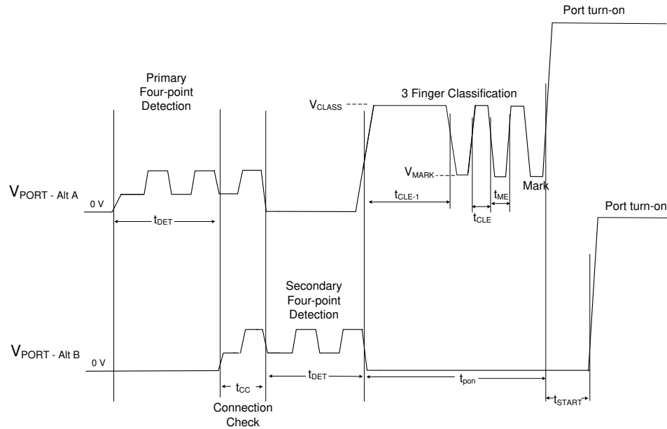
Figure 7-5. 4-Pair Single Signature Detection, 3-Event Classification and Turn On
