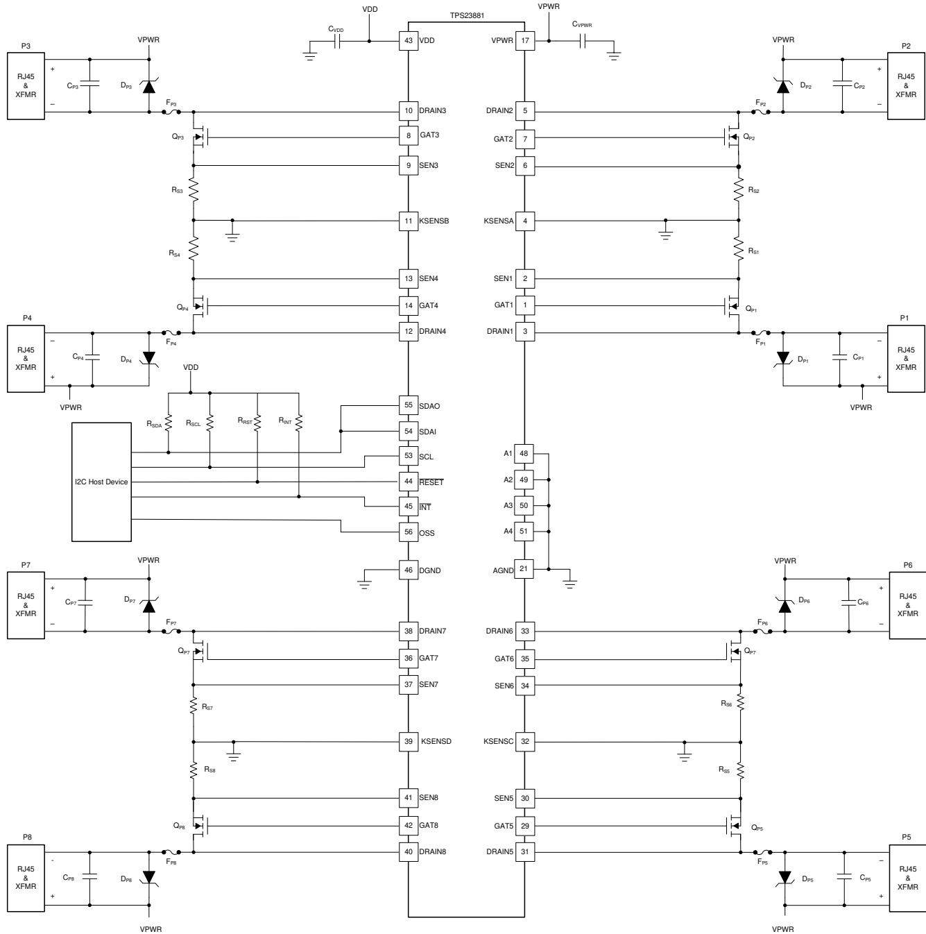
Figure 9-1. Eight 2-Pair Port Application
