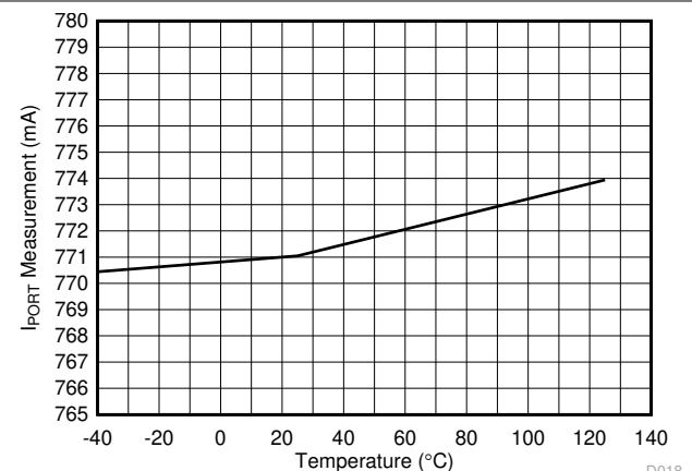
Figure 6-18. Port Current ADC Measurement (770mA) vs Temperature
