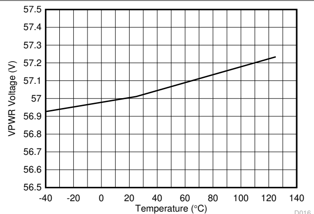
Figure 6-16. VPWR Voltage ADC Measurement vs Temperature
