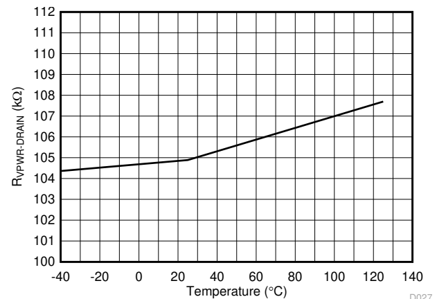
Figure 6-27. R_{\text{OFF}} (VPWR to DRAIN) vs Temperature
