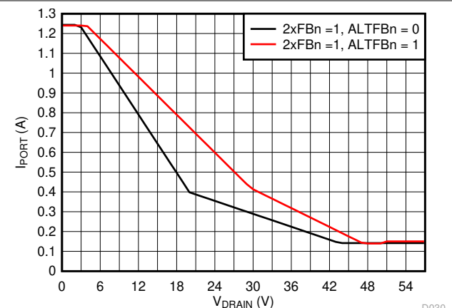
Figure 6-30. 2x Mode (2xFBn = 1) Current Foldback vs Drain Voltage
