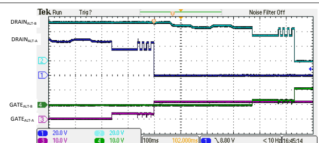
Figure 9-27. 4-Pair Dual Signature 4-Finger Classification and Turn On
