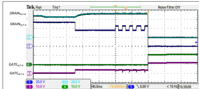
Figure 9-22. 4-Pair Single Signature 5-Finger Classification and Turn On
