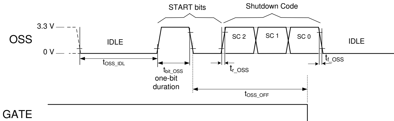
Figure 8-1. Multi Bit Priority Port Shutdown if Lower-Priority Port
