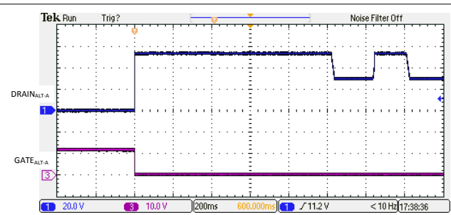
Figure 9-5. 2-Pair Backoff Due to PCut Fault
