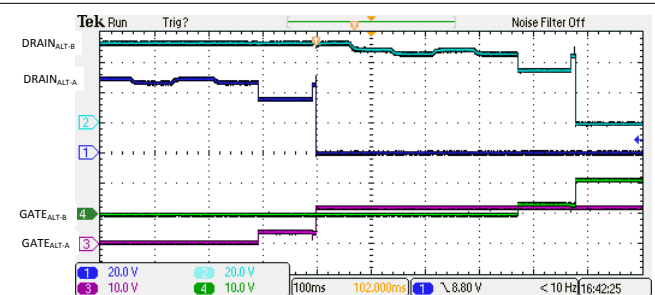
Figure 9-25. 4-Pair Dual Signature 1-Finger Classification and Turn On
