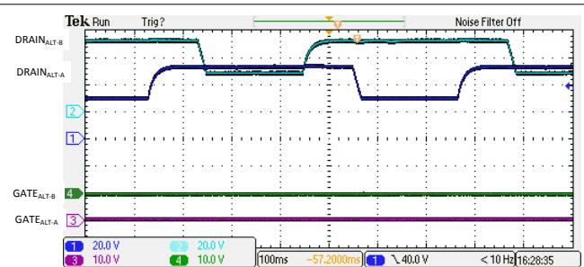
Figure 9-11. 4-Pair Open Circuit Detection Signature
