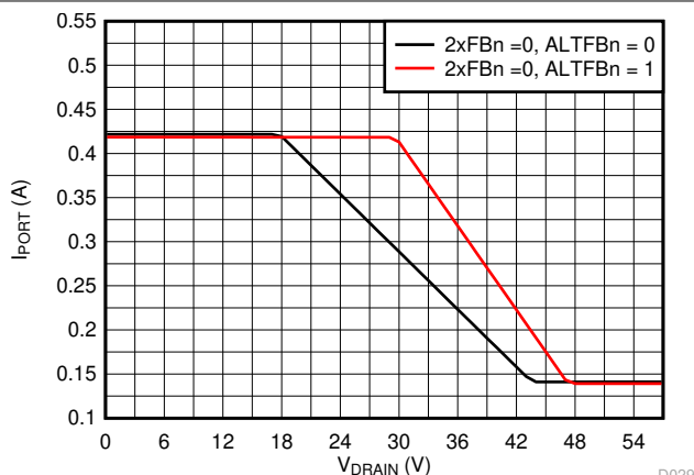
Figure 6-29. 1x Mode (2xFBn = 0) Current Foldback vs Drain Voltage
