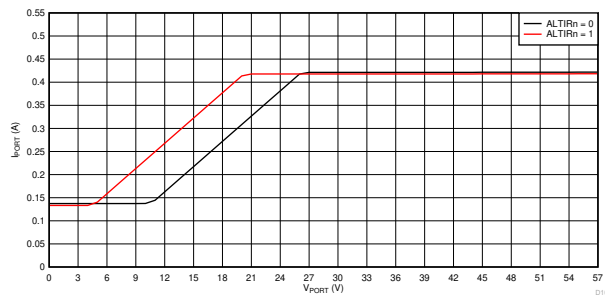
Figure 8-2. Foldback During Inrush (at Port Turn-On): I_{LIM} vs V_{port}
