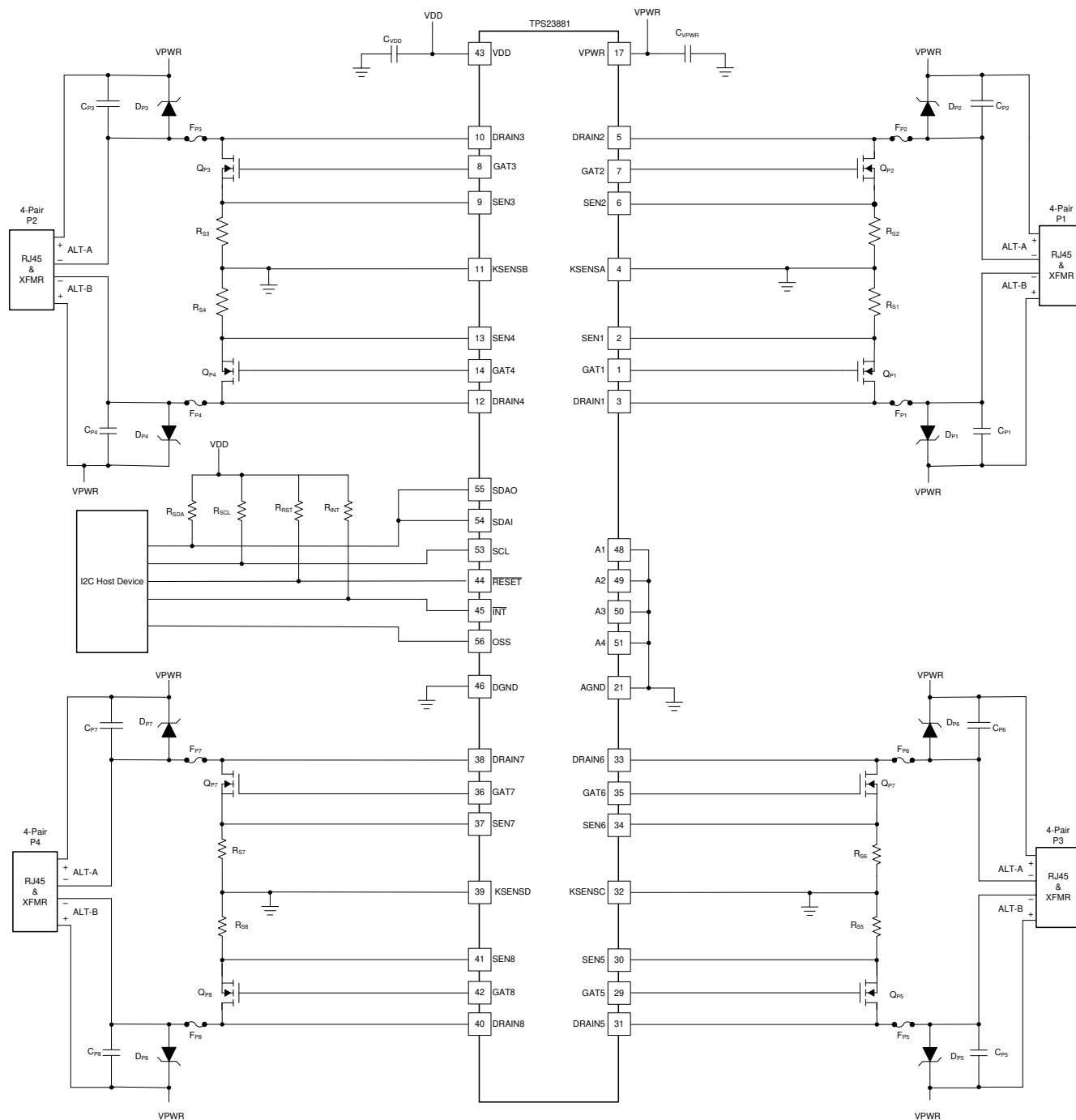
Figure 9-2. Four 4-Pair Port Application
