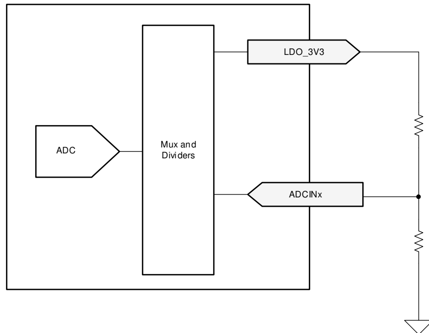
Figure 8-4. ADCINx Resistor Divider
