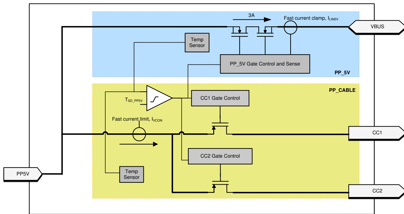
Figure 8-1. Port Power Switches
