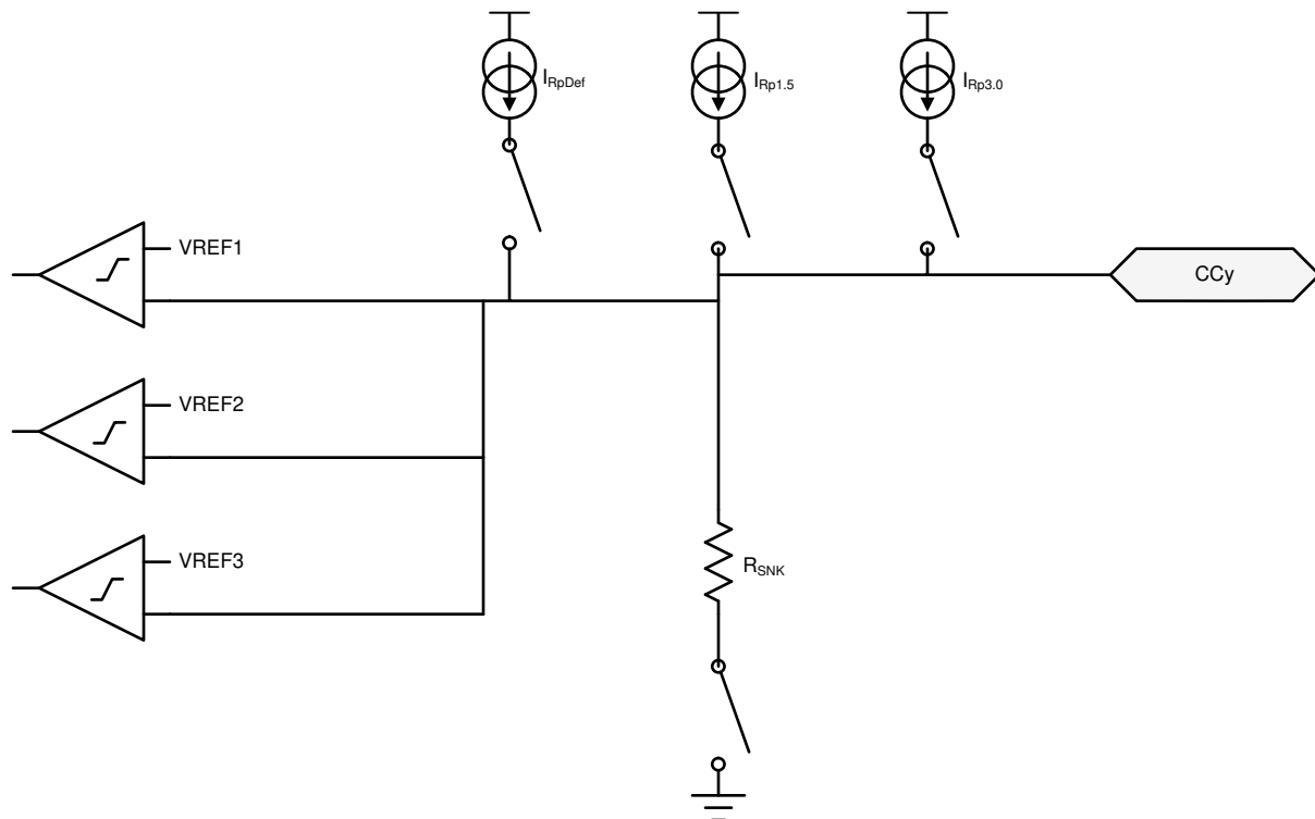
Figure 8-2. Plug and Orientation Detection Block
