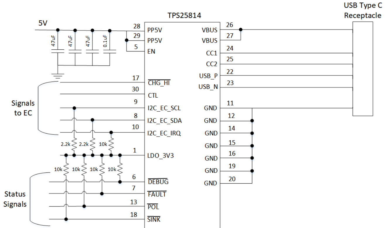
Figure 9-1. Type C DFP Port Implementation
