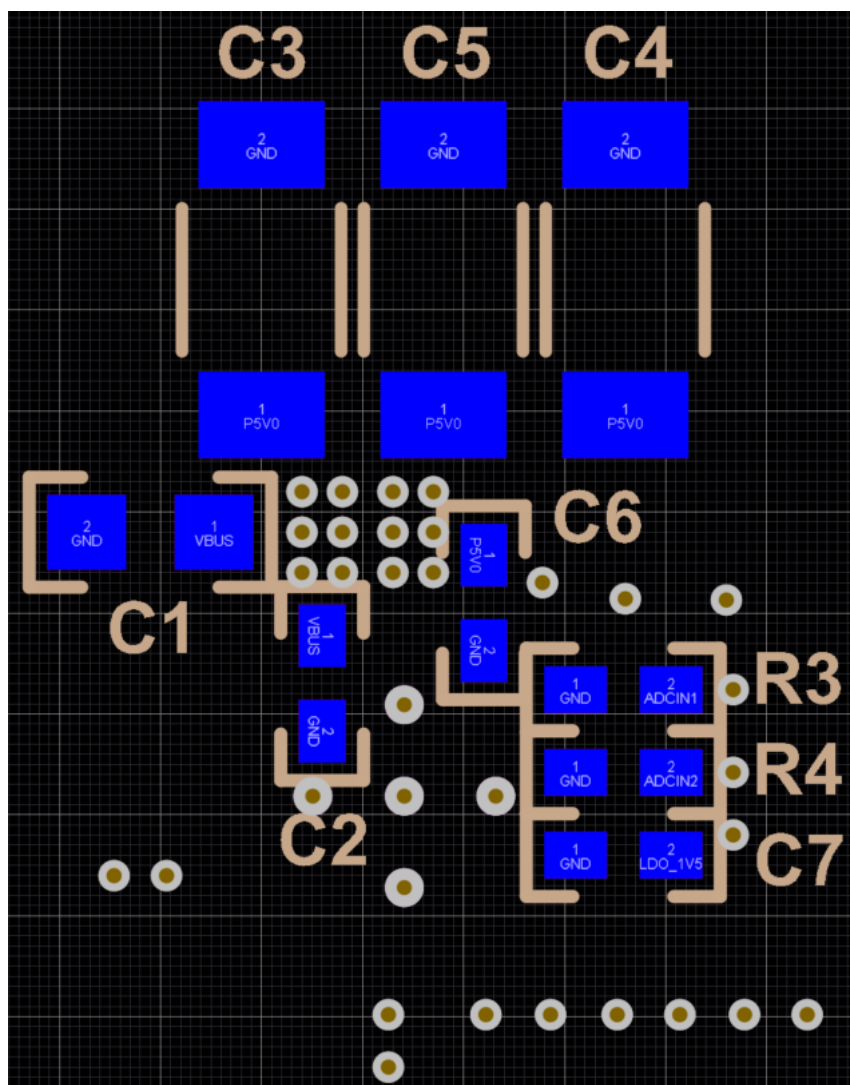
Figure 11-8. Via Placement - Bottom Layer
