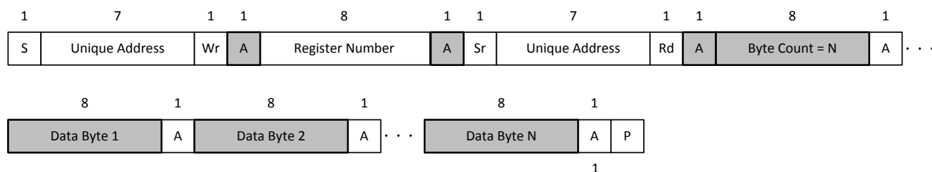
Figure 8-11. I 2 C Unique Address Read Register Protocol
