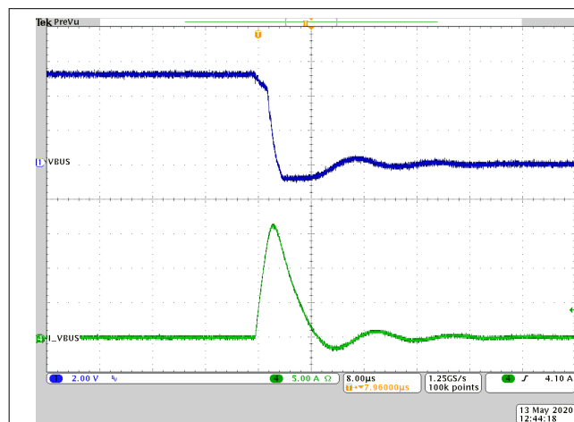
Figure 9-3. VBUS Short to Ground (Zoomed In)
