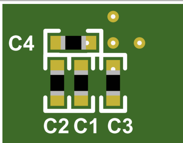
Figure 11-5. Bottom View 3-D
