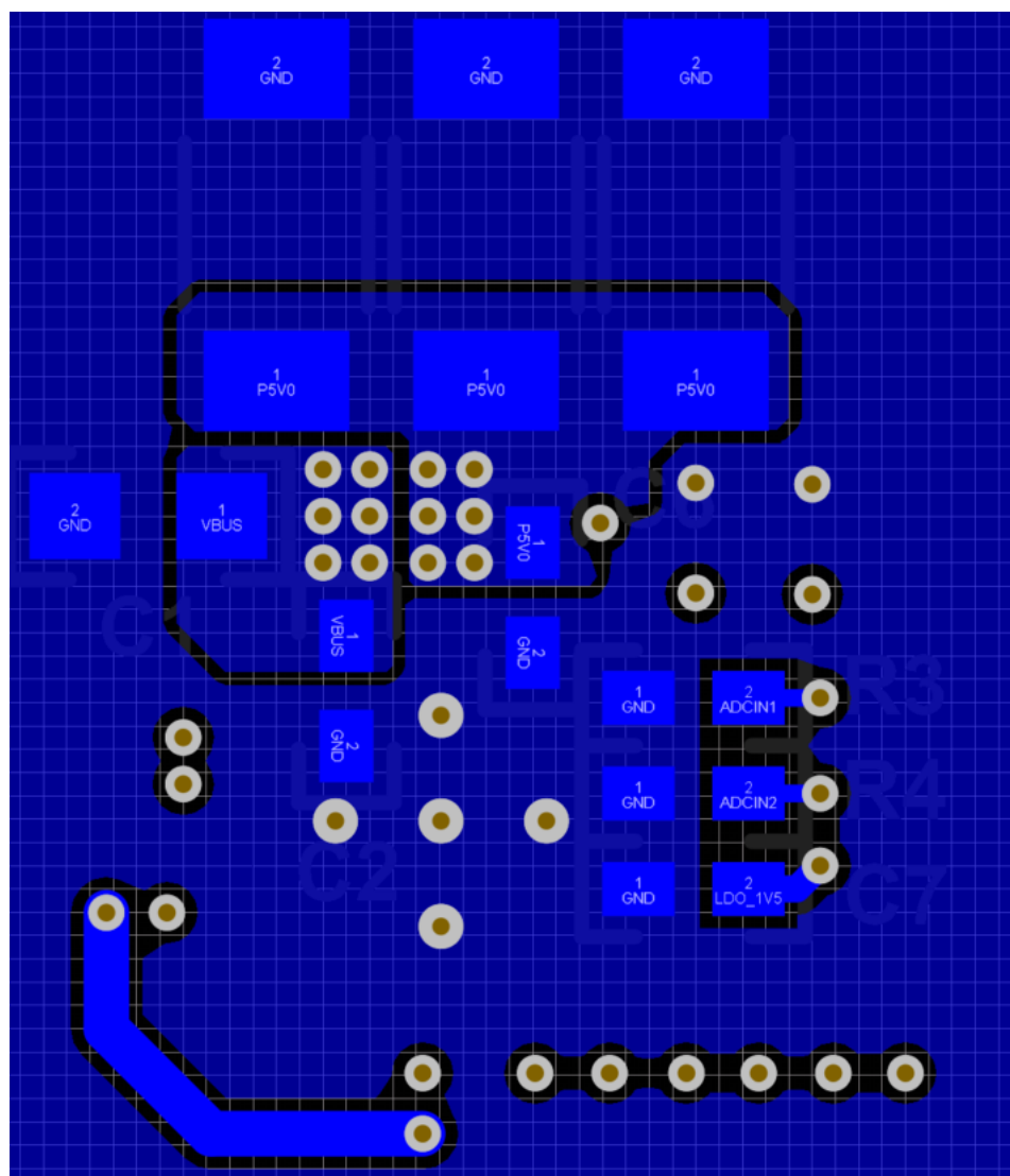
Figure 11-10. Routing - Bottom Layer
