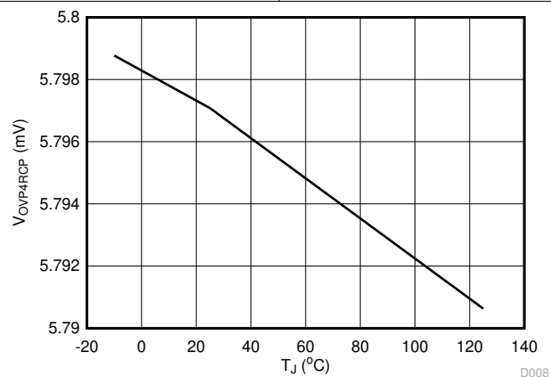
Figure 6-3. V OVP4RCP vs. Temperature
