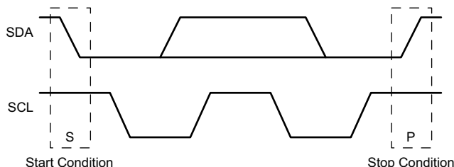
Figure 8-7. I 2 C Definition of Start and Stop Conditions
