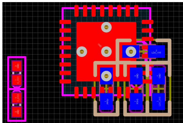
Figure 11-3. Bottom View Layout
