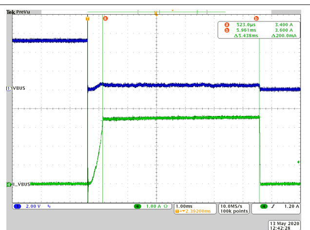
Figure 9-4. VBUS Short to Ground (Zoomed Out)
