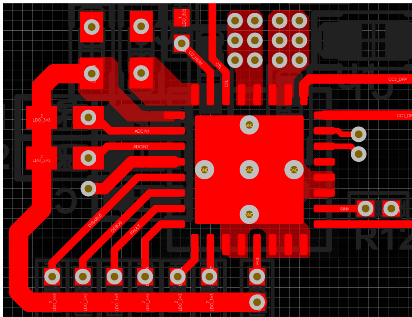
Figure 11-9. Routing - Top Layer
