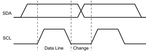
Figure 8-8. I²C Bit Transfer
