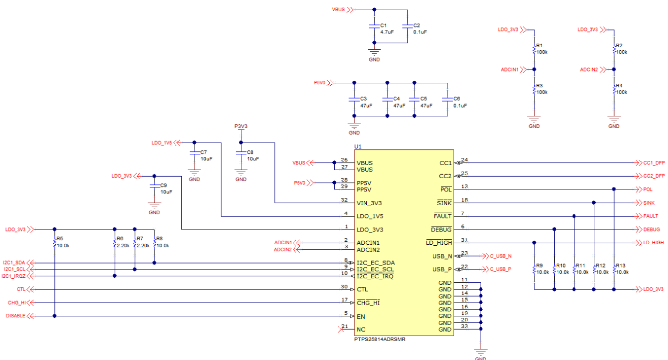
Figure 11-1. Example Schematic
