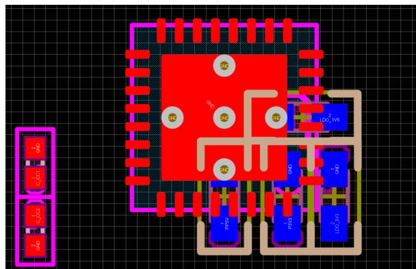
Figure 11-2. Top View Layout
