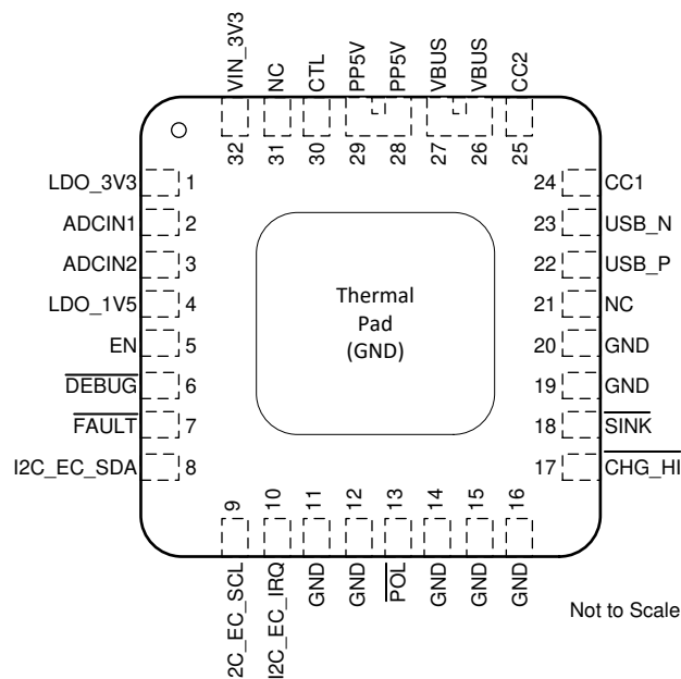
Figure 5-1. RSM Package 32-pin QFN Top View
