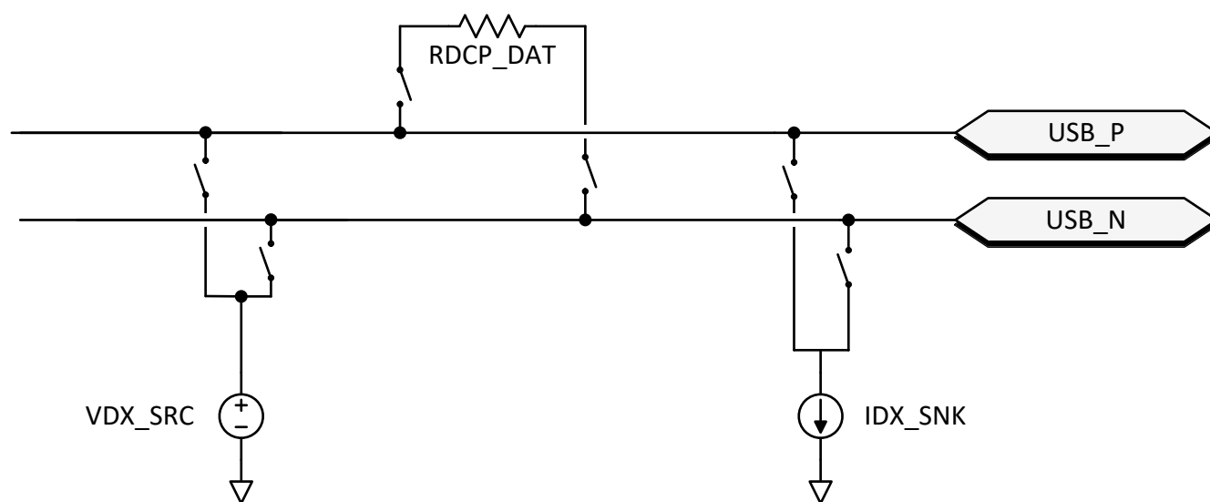
Figure 8-5. BC1.2 Hardware Components
