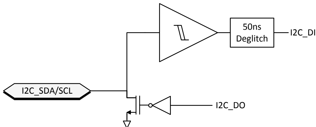
Figure 8-6. I 2 C Buffer
