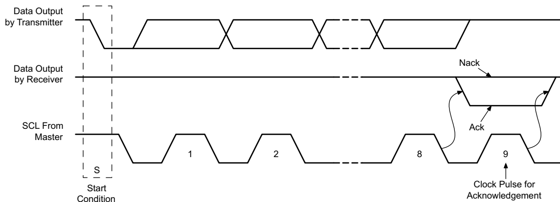
Figure 8-9. I²C Acknowledgment
