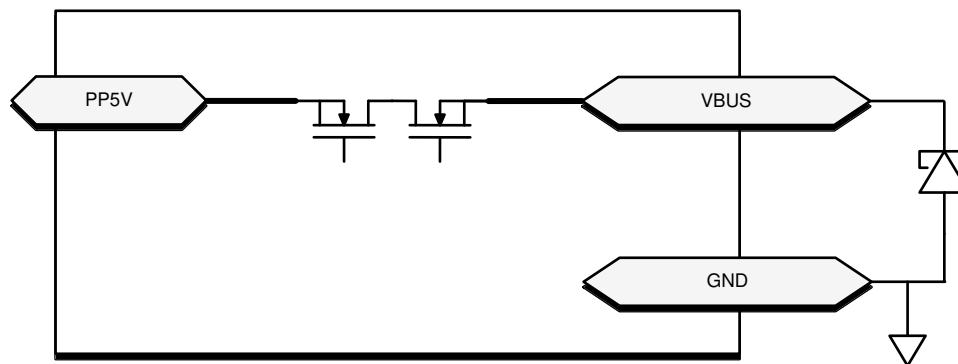
Figure 8-14. Schottky for Current Surge Protection
