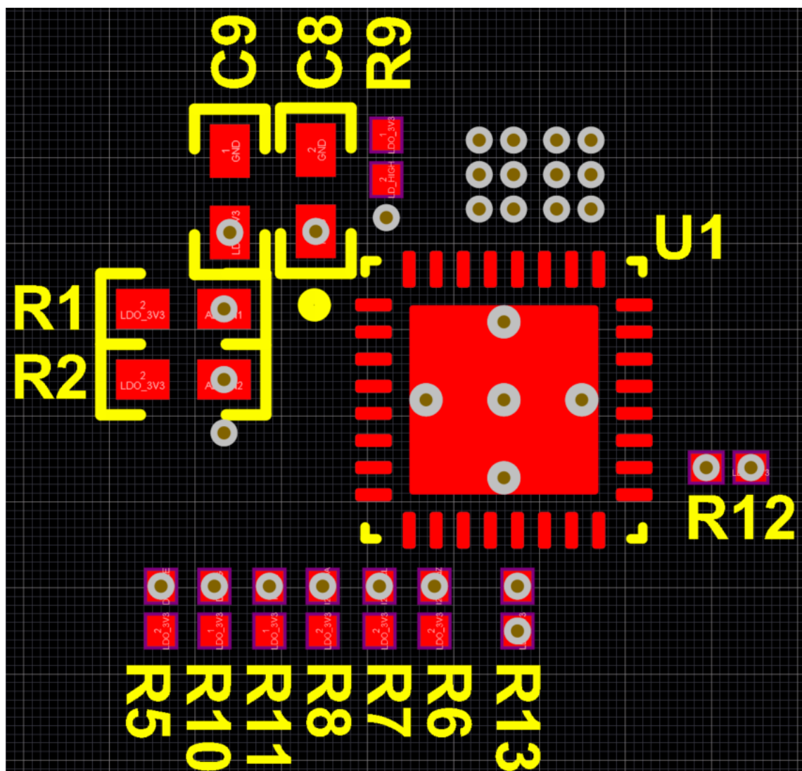
Figure 11-7. Via Placement - Top Layer
