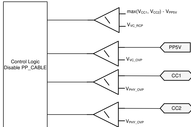
Figure 8-3. Overvoltage and Reverse Current Protection for CC1 and CC2
