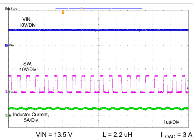
Figure 10-9. Switching Frequency When R_T = 8.87\text{ k}\Omega
