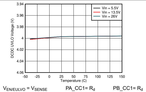
Figure 8-6. DCDC UVLO Threshold
