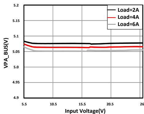
Figure 11-13. Dropout Characteristic
