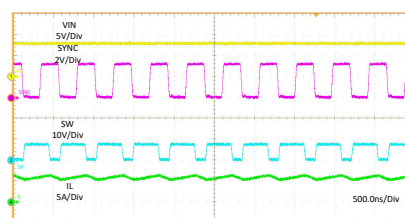
Figure 10-6. Switching Frequency When R_{FREQ} = 8.45 \text{ k}\Omega
