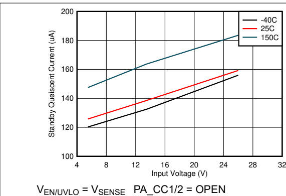
Figure 8-2. Standby Quiescent Current
