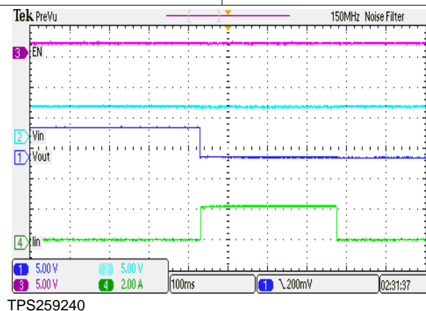
Figure 33. Short Circuit (Zoom): Fast-Trip Comparator
