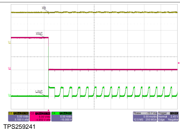
Figure 32. Transient: Output Short Circuit
