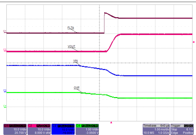
Figure 61. Overtoltage Recovery
