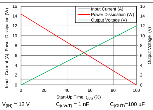
Figure 54. P_{D(INRUSH)} Due to Inrush Current
