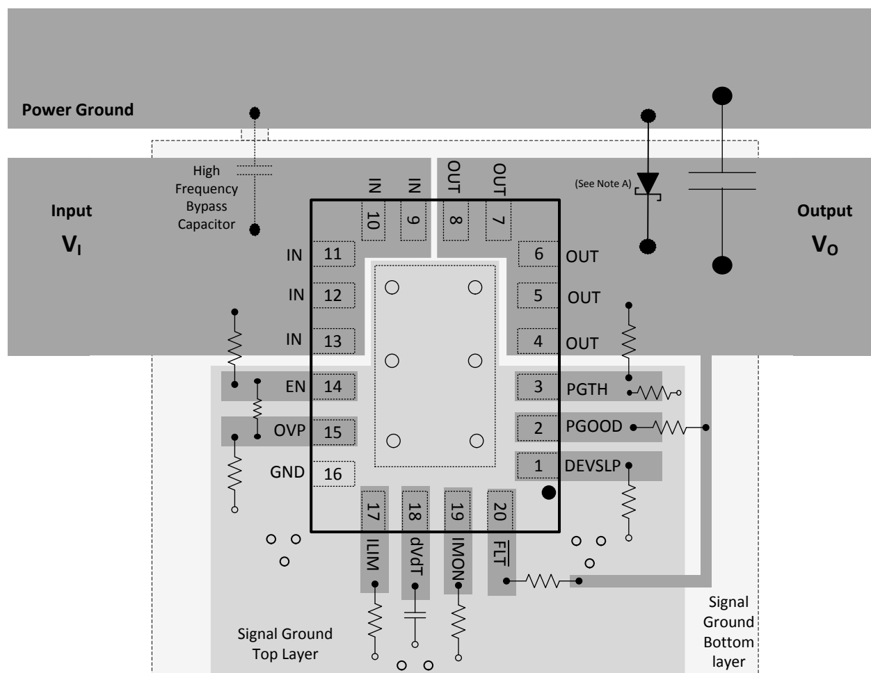
Figure 80. Board Layout
