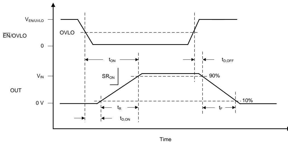
Figure 2. TPS2595x3 Switching Times
