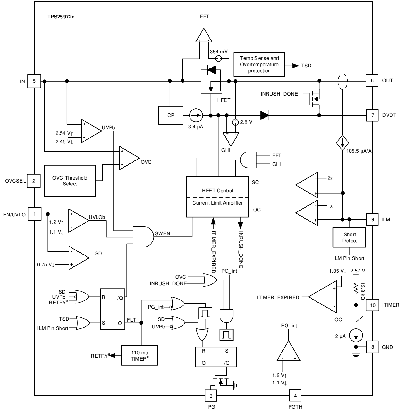
Figure 7-2. TPS25972x Block Diagram
