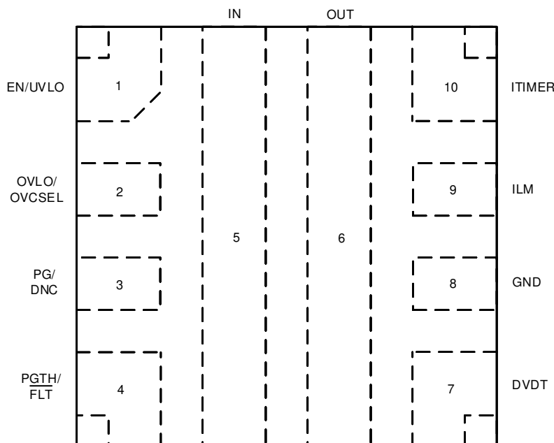
Figure 5-1. TPS2597xx RPW Package 10-Pin QFN (Top View)
