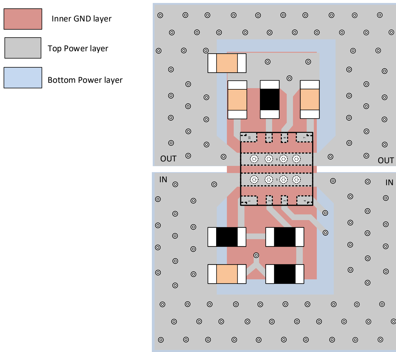
Figure 8-11. Layout Example - Single TPS25974x With PGTH Referred to OUT
