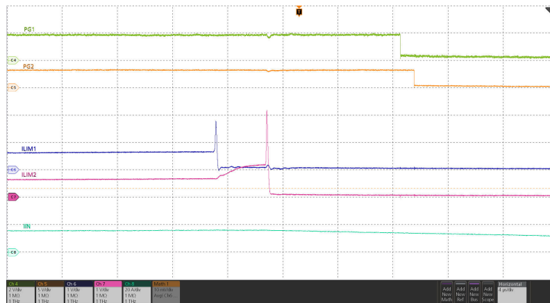
Figure 8-9. Parallel Devices Load Current During Steady State and Overload
