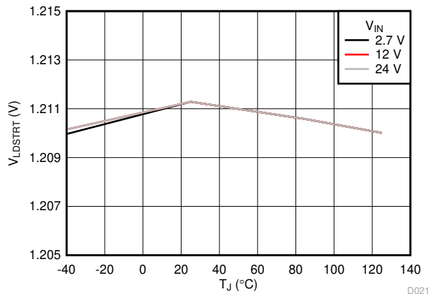
Figure 6-16. LDSTRT Threshold Voltage vs Temperature
