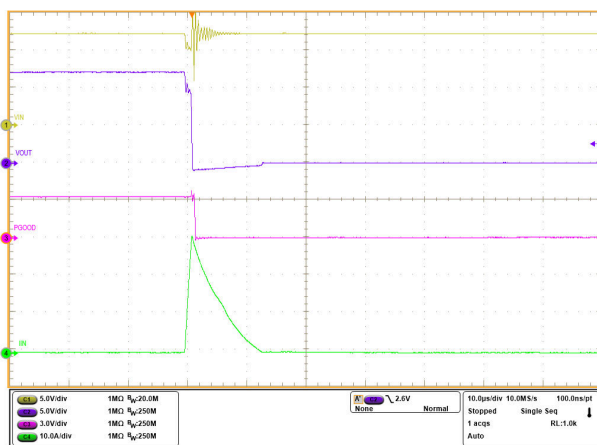
Figure 6-30. Power Up Into Output Short-Circuit
