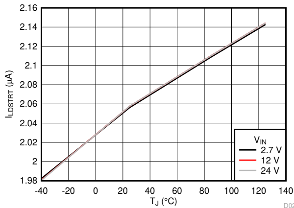
Figure 6-15. LDSTRT Charging Current vs Temperature
