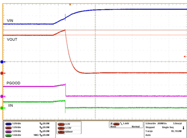
Figure 8-19. Overvoltage Cut-off at 3.7V with TPS2598020 Device
