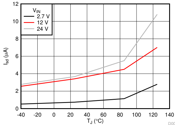
Figure 6-9. Deep Shut-Down Current vs Temperature
