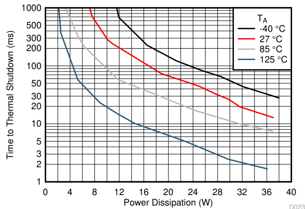
Figure 6-22. Thermal Shutdown Plot - Steady State
