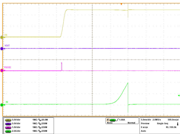
Figure 6-28. Circuit Breaker With Transient Overcurrent Blanking
