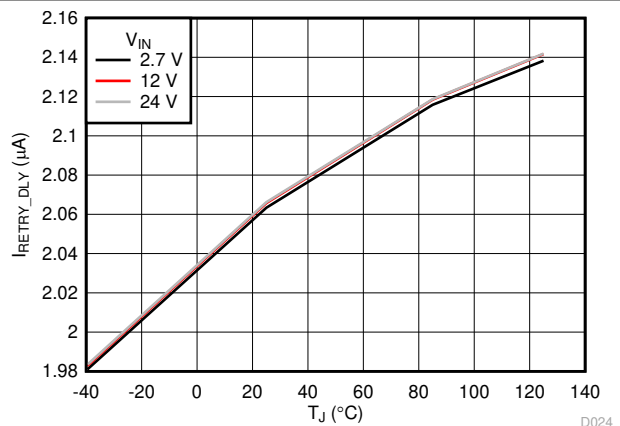
Figure 6-18. RETRY_DLY Bias Current vs Temperature
