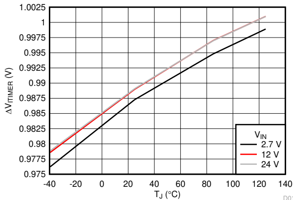
Figure 6-13. ITIMER Voltage Threshold Delta vs Temperature
