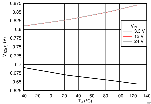
Figure 6-7. EN/UVLO Falling Threshold for Lowest Current Consumption
