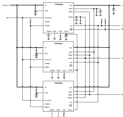
Simplified schematic
