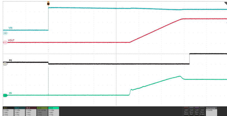
Figure 8-2. Insertion Delay
