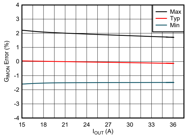
Figure 7-10. IMON Gain Accuracy Across Process and Temperature Corners
