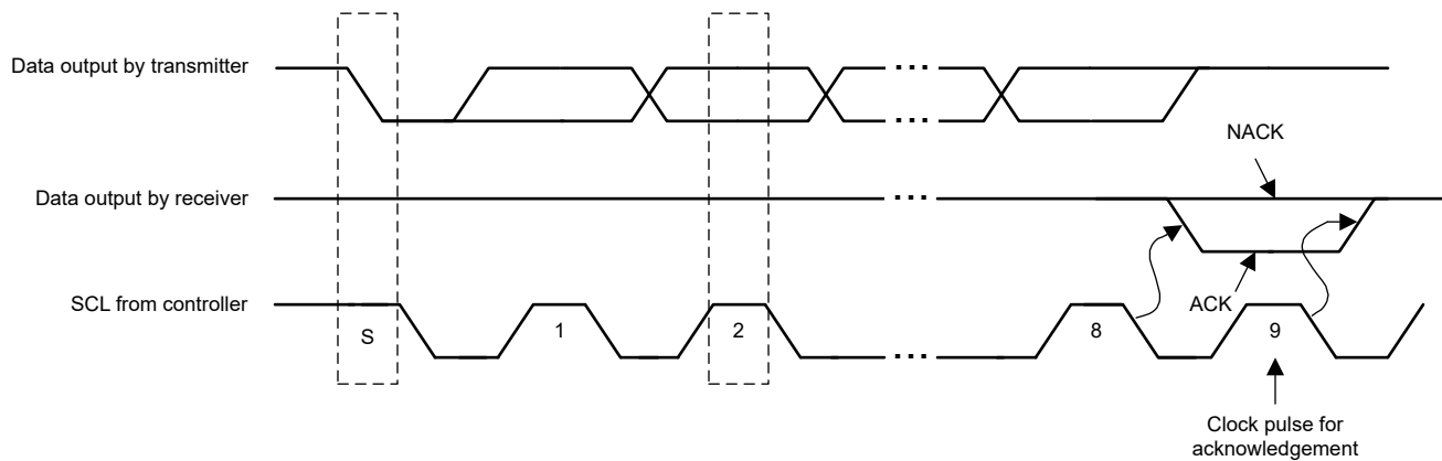
Figure 8-32. I²C Acknowledgment
