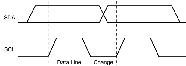
Figure 8-31. I²C Bit Transfer
