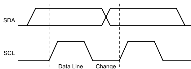
Figure 8-30. I 2 C Bit Transfer
