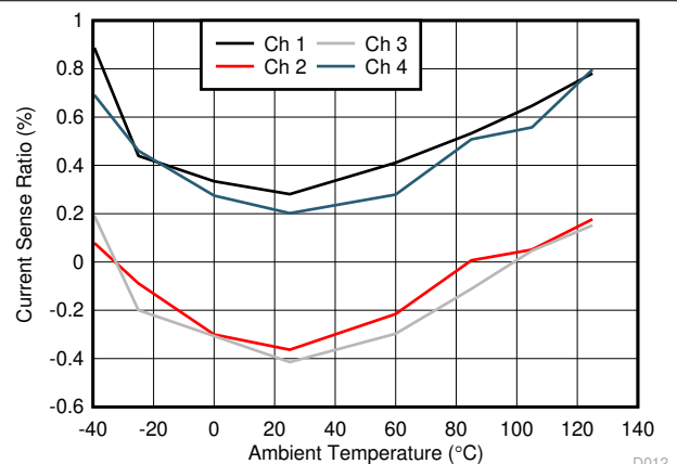
Figure 7-16. Current-Sense Ratio at 50 mA
