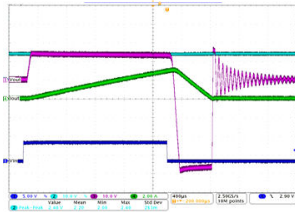
Figure 8-7. Inductive Load Switching-Off Waveform
