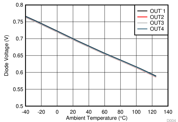
Figure 7-8. Body-Diode Forward Voltage
