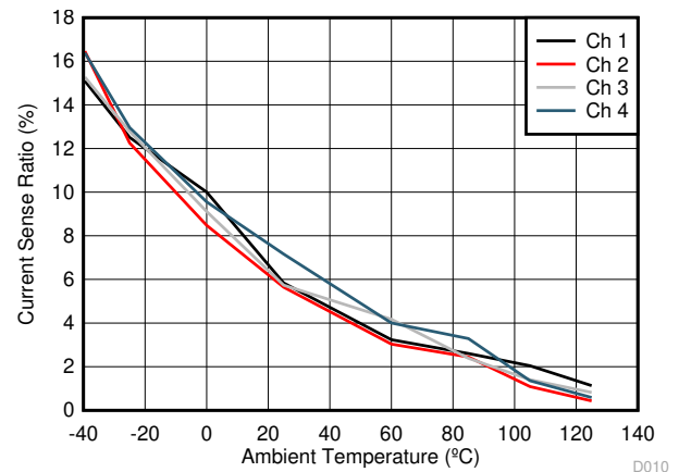
Figure 7-14. Current-Sense Ratio at 5 mA
