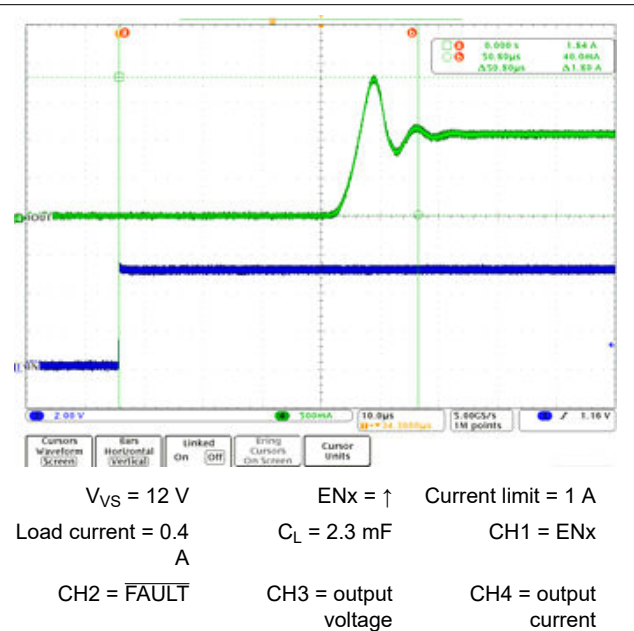
Figure 9-4. Driving a Capacitive Load, Expanded Waveform
