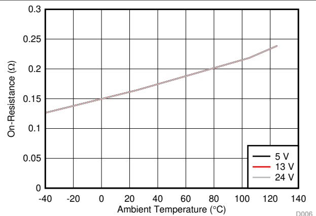
Figure 7-10. Channel-1 FET On-Resistance
