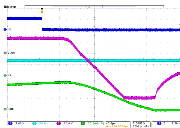
Figure 29. Inductive Load Switching-Off Expanded Waveform
