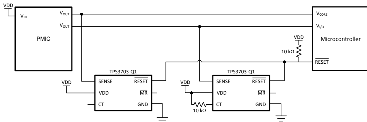
Figure 9-6. Two TPS3703-Q1 Monitoring Two Microcontroller Power Rails
