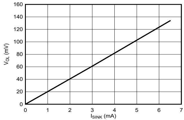
Figure 6-10. Open-Drain Active Low V_{OL} vs I_{RESET} ( V_{DD} = 65\text{ V} )
