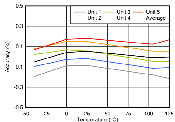
Overvoltage Threshold ( V_{IT+(OV)} ) Accuracy vs Temperature
