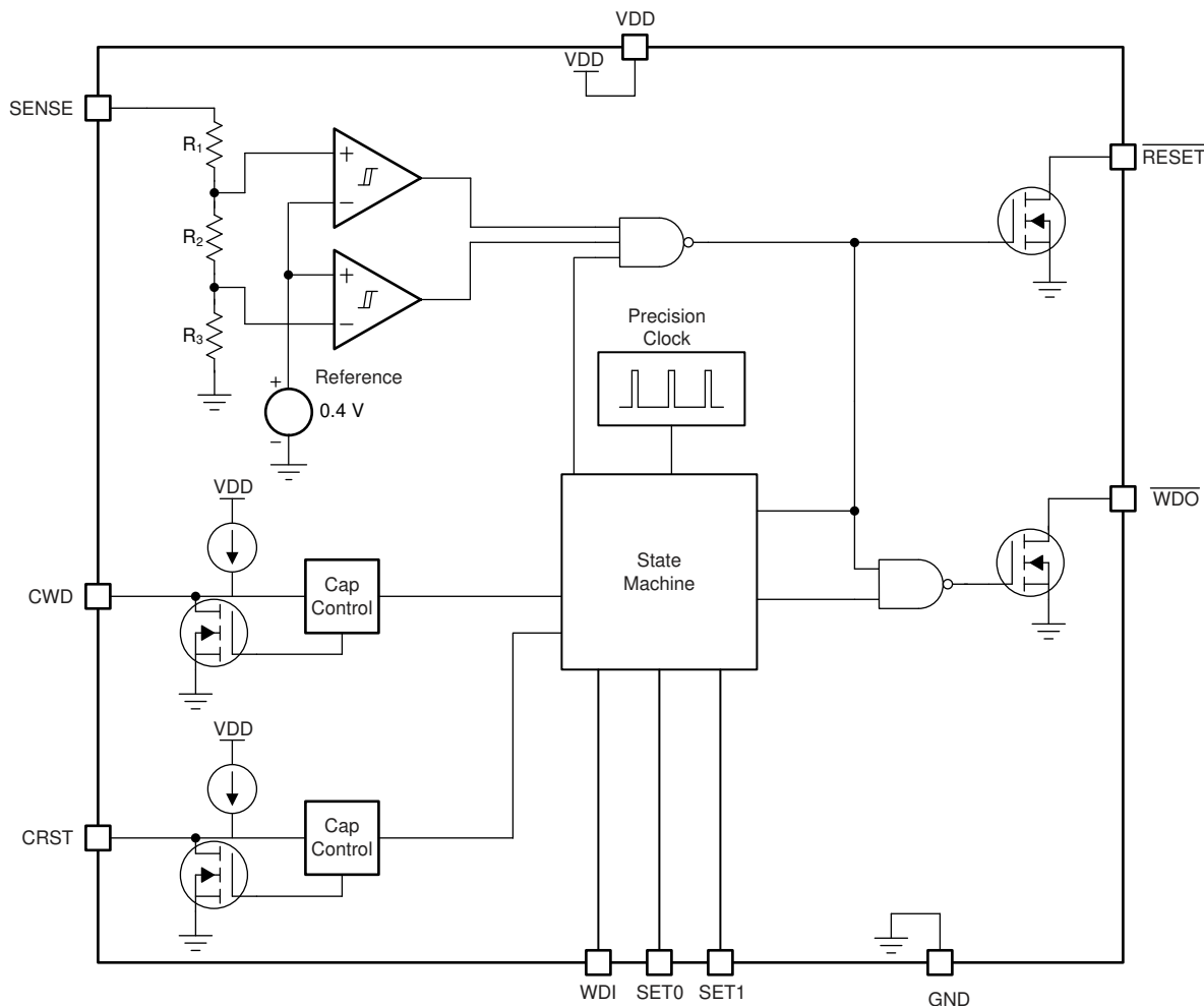
Figure 7-1. Fixed Version Block Diagram
