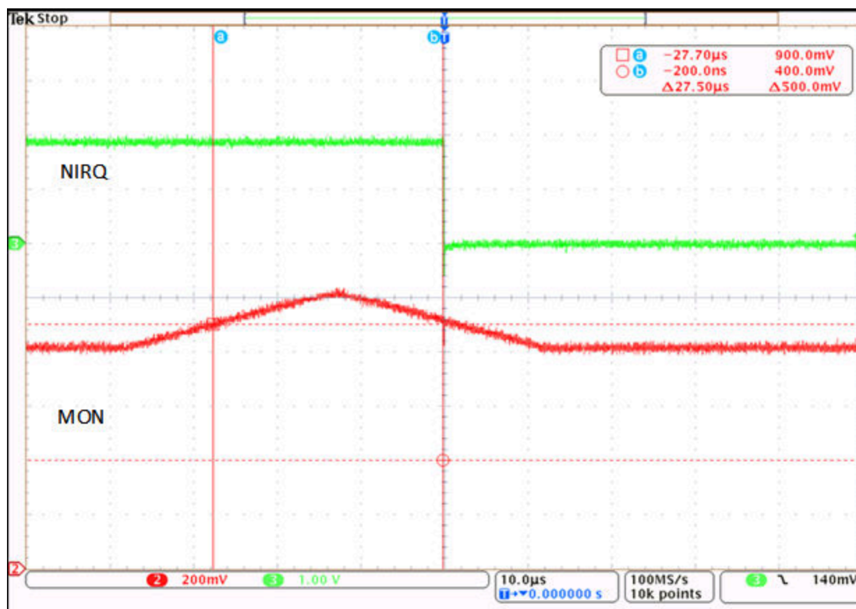
Figure 8-7. NIRQ Triggered on Overvoltage Fault with 25µs OV Debounce Filter
