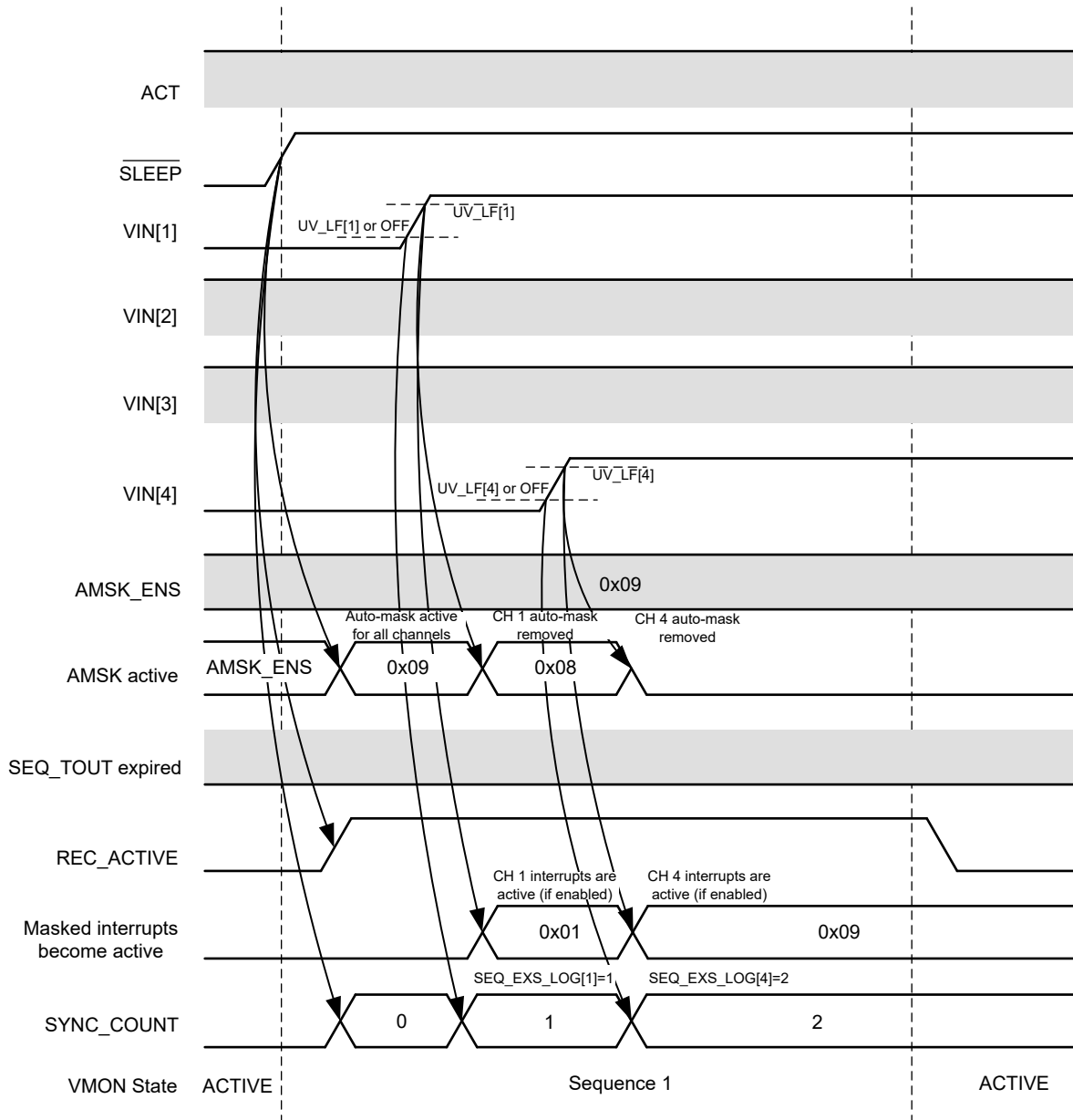
Figure 7-16. SLEEP 0→1 Transition
