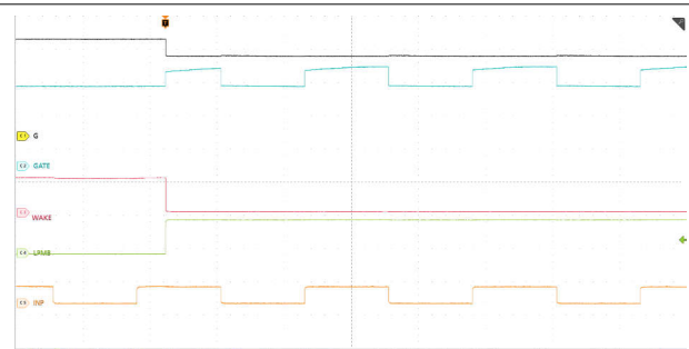
Figure 9-7. With \overline{\text{LPM}} = Low to High, \text{INP} Gained Control on \text{GATE} ( V_{\text{IN}} = 48V, No Load)
