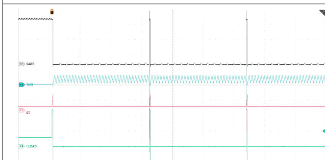
Figure 9-10. Auto-Retry Response of TPS4812-Q1 for an \text{I}^2\text{T} -Based Overcurrent Fault
