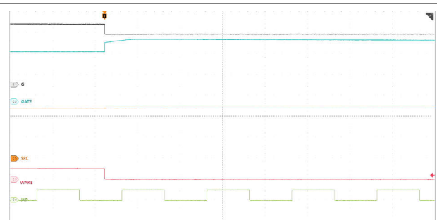
Figure 9-5. When \overline{\text{LPM}} = Low in LOAD WAKEUP state, \text{INP} Has No Control on \text{GATE}
