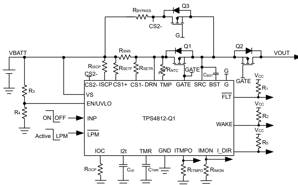
Figure 9-1. TPS4812-Q1 Application circuit for driving power at all times (PAAT) loads with automatic load wakeup
