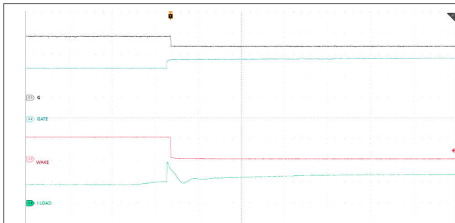
Figure 9-4. Zoom-In View of State Transition From LPM to Active Mode ( \overline{\text{LPM}} = Low, V_{\text{IN}} = 48V, \text{EN/UVLO} = High)
