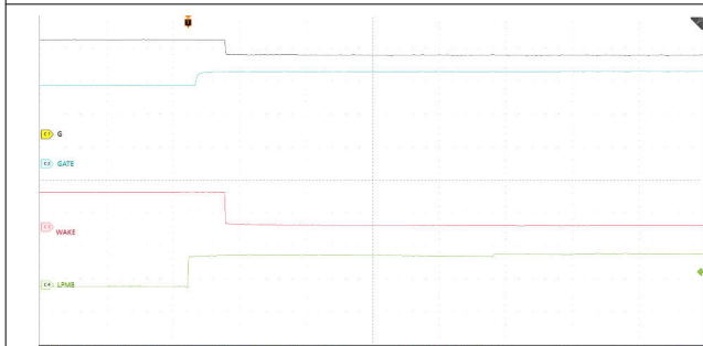
Figure 9-6. State Transition From LPM to Active Mode ( \overline{\text{LPM}} = Low to High, V_{\text{IN}} = 48V, No Load)
