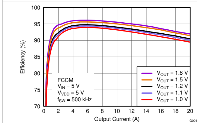
Figure 6-32. Efficiency vs Output Current
