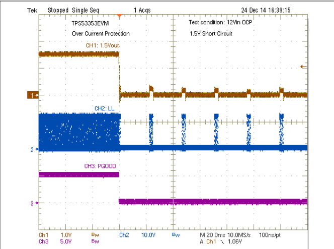
Figure 8-12. Output Short-Circuit Protection
