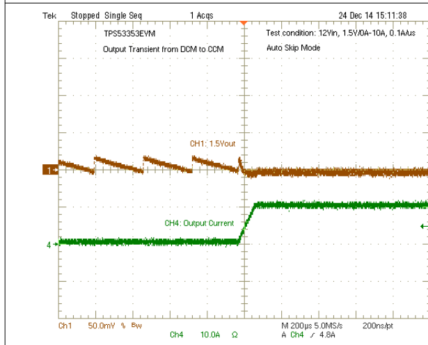
Figure 8-7. Output Transient from DCM to CCM
