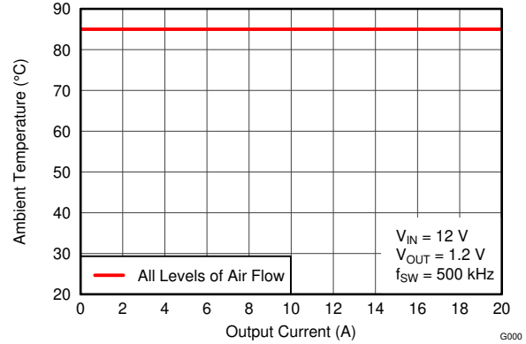
Figure 6-26. Safe Operating Area
