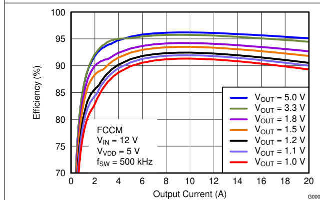
Figure 6-30. Efficiency vs Output Current
