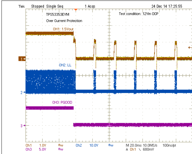
Figure 8-11. Output Overcurrent Protection
