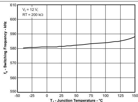
Figure 4. Switching Frequency vs Junction Temperature
