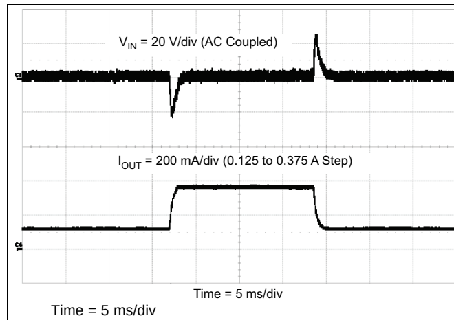
Figure 51. Load Transient
