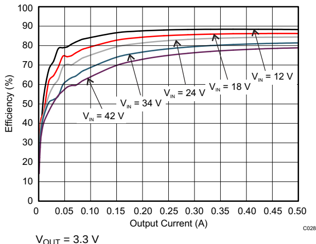
Figure 58. Efficiency vs Load Current
